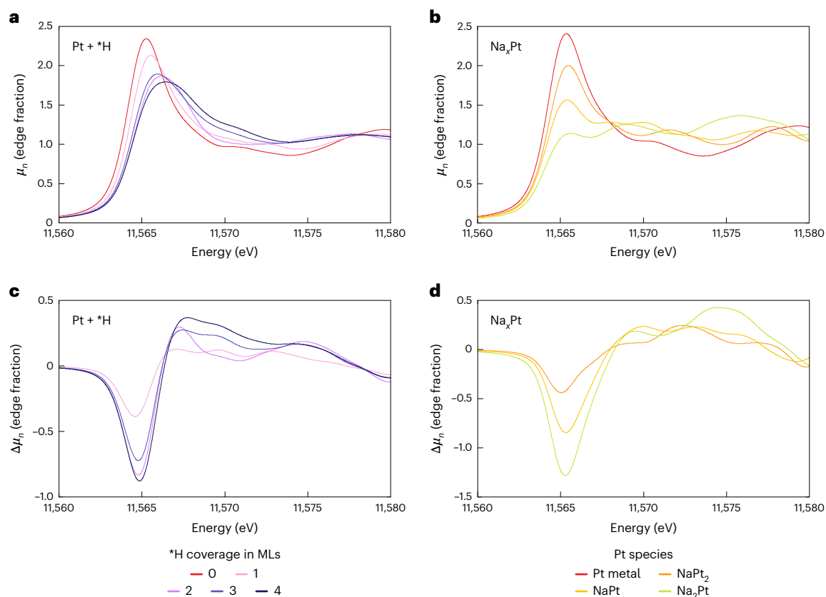
Fig. 1 | OCEAN-based spectra for hydrogen-covered platinum and bulk platinumides. a,c, Theoretical first-principles calculations of Pt L_{III} edge X-ray absorption spectra of platinum with zero through four MLs of *H on Pt(111) (a), and corresponding difference spectra that are obtained by subtracting the
