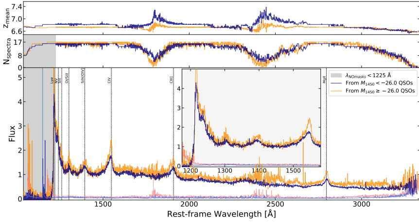
Figure 2.8: Bottom panel: Composite spectrum of the 16 spectra having M_{1450} < -26.0 (dark blue curve), compared with the composite spectrum obtained from the 17 spectra with M_{1450} \geq -26.0 (orange curve); where M_{1450, \text{median, non-BAL}} = -26.0 is the median M_{1450} of the 33 non-BAL quasars. The rest of the plot shows the same quantities already described in Fig. 2.5.
