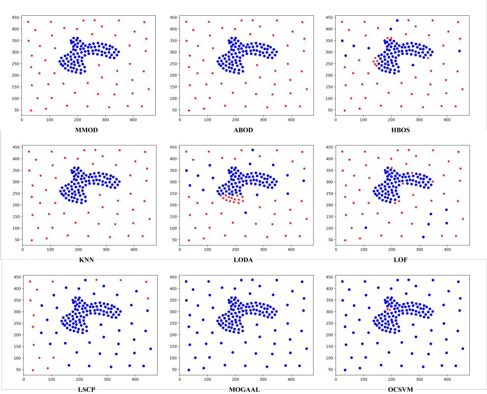
Figure 5.9: Nine algorithms’ outlier detection results on the synthetic “Uniform outliers” dataset. Detected outliers are in red.
