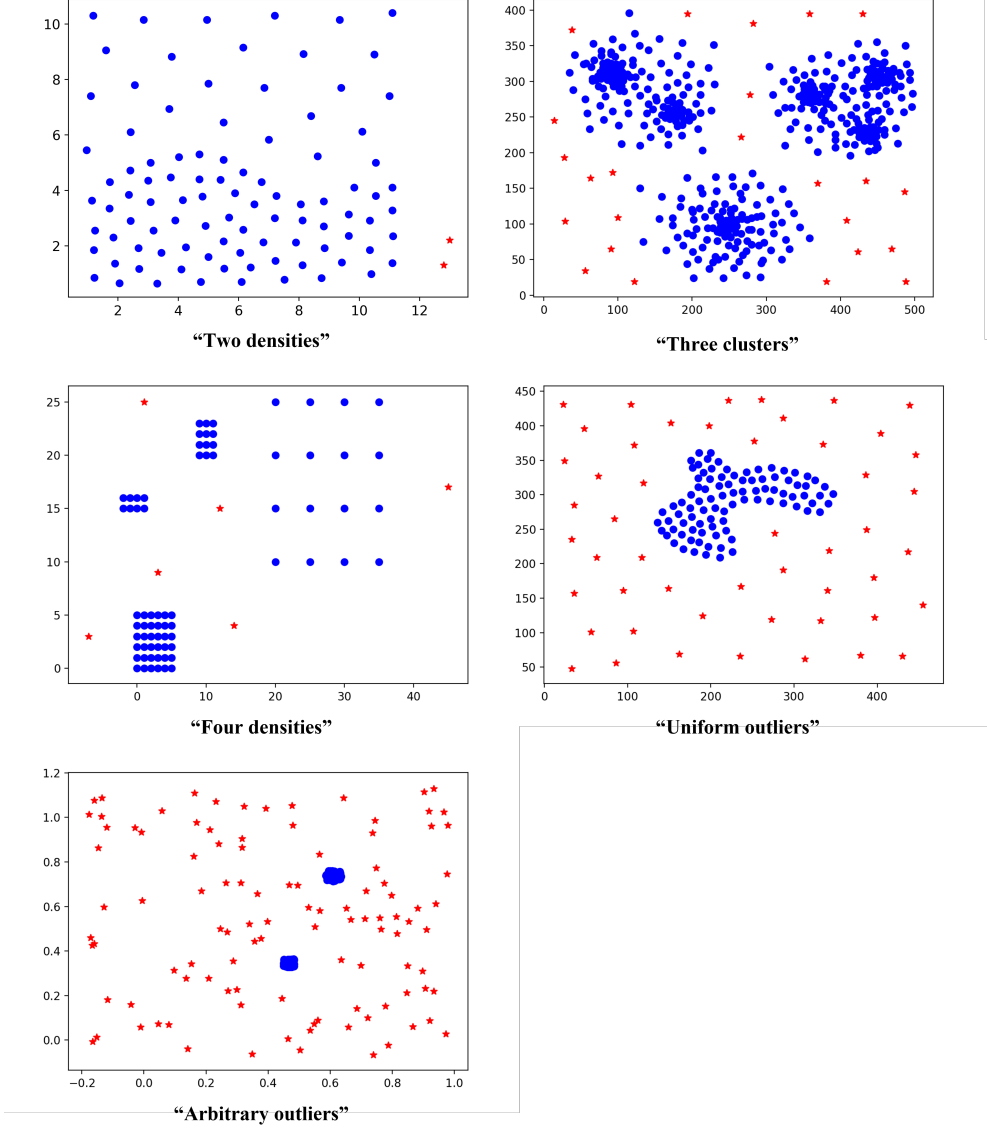
Figure 5.5: Summary of MMOD's outlier detection results on the five synthetic two-dimensional datasets. Red: outliers detected by the proposed adaptive minimum spanning tree-based outlier detection (MMOD) method.
