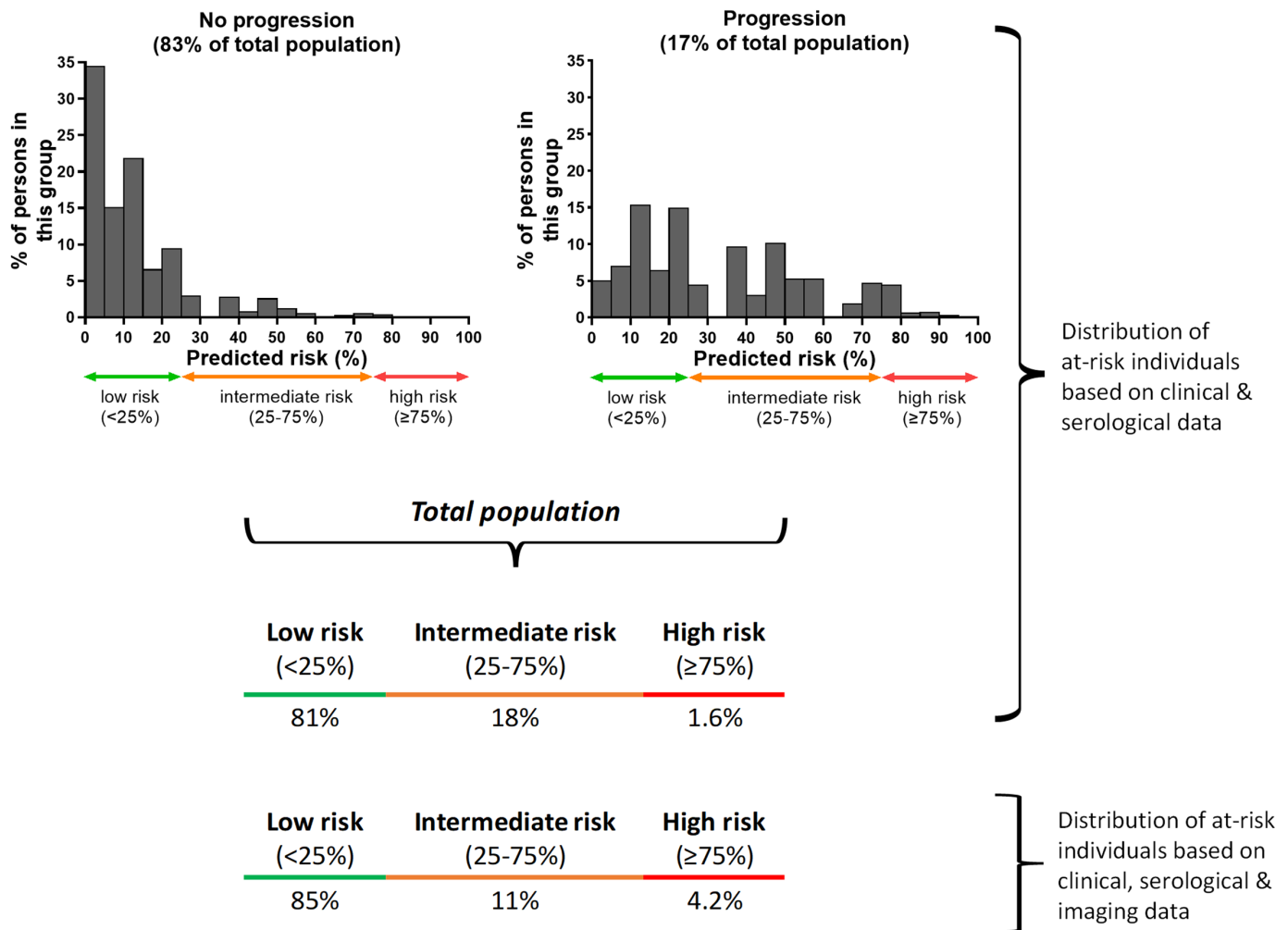
Figure 3. Distribution of subjects who did not and did reach the endpoint based on the predicted risks using the risk stratification criteria with clinical and serologic data in Table 4. Subsequently, risk categories were defined as low (<25% risk), intermediate (25%-75%) and high (≥75%) in the total population based on clinical and serologic data ( n = 2,293 ). The same was done when additionally using MRI data ( n = 703 ). Characteristics of persons who developed the endpoint and were categorized as low risk (8% of the total population) are presented in Supplemental Table S10, both for the setting without and with imaging data. MRI, magnetic resonance imaging.
