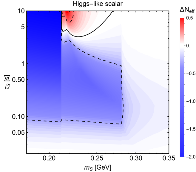
FIG. 3. Effect of Higgs-like scalars on \Delta N_{\text{eff}} in the parameter space of the scalar mass m_S and lifetime \tau_S . The solid black line marks the parameter space where \Delta N_{\text{eff}} = 0 , while dashed lines indicate regions where \Delta N_{\text{eff}} exceeds the Planck 95% CL bound [45]. Similarly to the bottom panel of Fig. 2, the plots have been obtained using the unintegrated neutrino Boltzmann solver. In the mass range 2m_\mu < m_S < 2m_\pi , \Delta N_{\text{eff}} experiences the transition between negative and positive values (as in Fig. 2).
