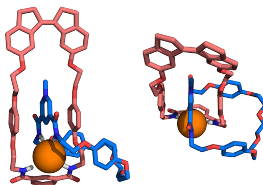
Fig. 1 Front- and top-views of catenane (Z)-1-Cl as found in the crystal structure, shown in a capped stick representation. Disorder in the oligo-ethylene glycol part of the pyridinium macrocycle has been omitted for clarity.
