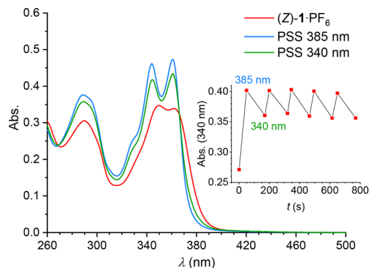
Fig. 2 UV-vis spectral changes of (Z)-1-PF 6 upon consecutive irradiation with 385 nm and 340 nm light ( c = 2.0 \times 10^{-5} M in dry and degassed DMSO) and change in absorption at 340 nm during 385/340 nm irradiation cycles (inset).
