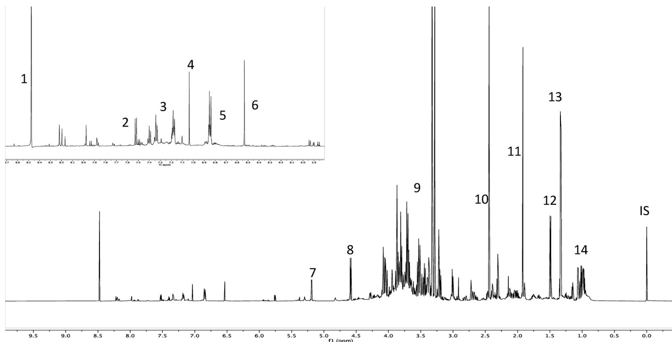
Fig. 2. ^1\text{H} -NMR of Barley extract. Barley was extracted with hot water (60°C for 2 h) and measured in MeOD- \text{D}_2\text{O} phosphate buffer at pH 6 as described in the method section 2.4.
