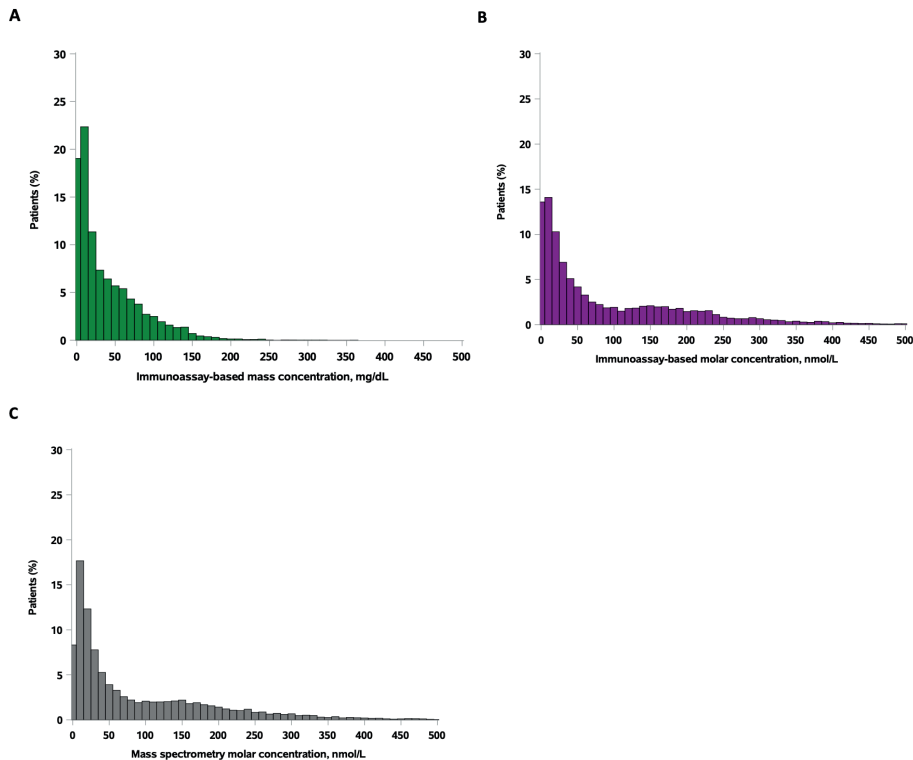
Figure S1: Histogram of baseline lipoprotein(a) concentrations for all patients in the analysis cohort: (A) Immunoassay-based mass concentration; (B) Immunoassay-based molar concentration; (C) Mass spectrometry molar concentration. Median (IQR) overall baseline concentrations were 21.8 (6.9, 60.0) mg/dL for IA-mass, 45.0 (13.2, 153.8) nmol/L for IA-molar, and 42.2 (14.3, 143.1) nmol/L for MS. IA indicates immunoassay.
