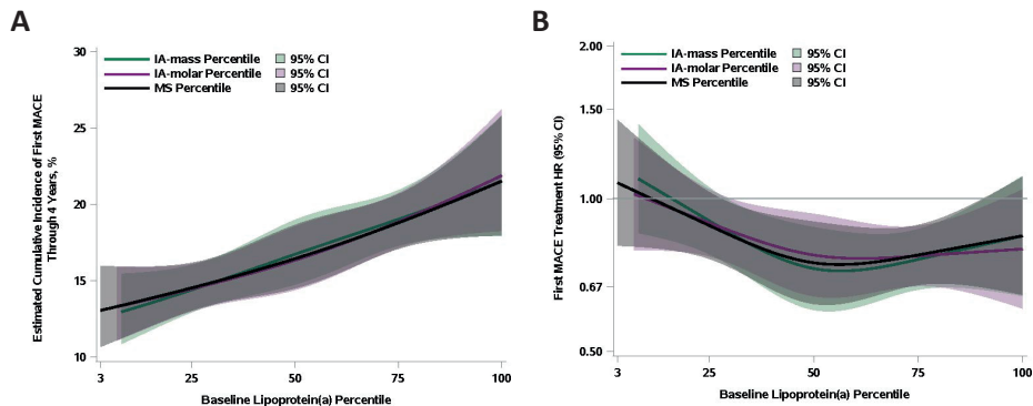
Figure 2: Spline analysis of risk of first MACE event by baseline lipoprotein(a) concentration percentiles. A, Cumulative incidence of first major adverse cardiovascular event (MACE) through 4 years within the placebo group. B, First MACE alirocumab:placebo hazard ratio. Splines are natural cubic with knots specified at the 25th, 50th, and 75th percentiles and reflect adjustment for baseline low-density lipoprotein cholesterol (LDL-C). Within the placebo group, spline P=0.0001 , 0.0002 , and 0.0003 for immunoassay-based mass test (IA-mass), immunoassay-based molar test (IA-molar), and mass spectrometry (MS), respectively, adjusted for LDL-C; spline P<0.0001 , P<0.0001 , and P=0.0001 for IA-mass, IA-molar, and MS, respectively, adjusted for LDL-C, age, sex, race, body mass index, history of diabetes, and triglycerides; all spline \times LDL-C interactions P>0.10 . Treatment \times spline interaction P=0.0474 , 0.21 , and 0.16 for IA-mass, IA-molar, and MS, respectively, adjusted for LDL-C. HR indicates hazard ratio.
