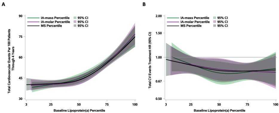
Figure S5: Spline analysis of total cardiovascular events by baseline lipoprotein(a) concentration percentiles: (A) Total cardiovascular events per 100 patients through 4 years within the placebo group; (B) total cardiovascular events alirocumab:placebo hazard ratio. Splines are natural cubic with knots specified at the 25 th , 50 th , and 75 th percentiles and reflect adjustment for baseline LDL-C corr . All spline P < 0.0001 adjusted for LDL-C corr and spline P = 0.0007 , 0.0003, and 0.0011 for IA-mass, IA-molar, and MS, respectively adjusted for LDL-C within the placebo group. All spline \times LDL-C corr and spline \times LDL-C interaction P > 0.10 within the placebo group. All treatment \times spline interaction P > 0.10 adjusted for LDL-C corr and P > 0.10 adjusted for LDL-C. CI indicates confidence interval; CV, cardiovascular; IA, immunoassay; LDL-C, low-density lipoprotein cholesterol; LDL-C corr , corrected low-density lipoprotein cholesterol; MS, mass spectrometry; HR, hazard ratio.
