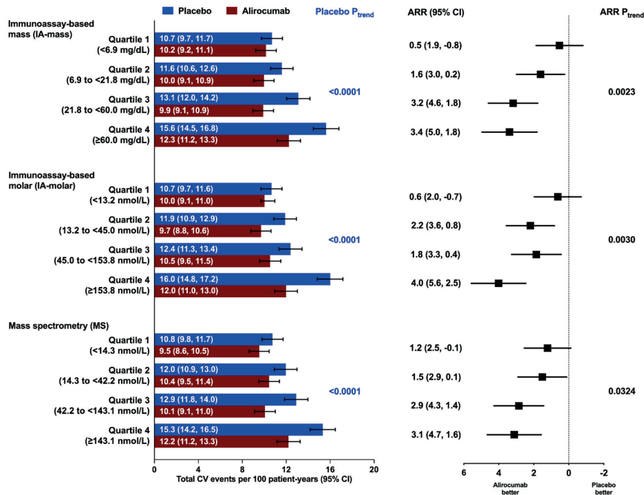
Figure S6: Rates of total cardiovascular events and absolute rate reductions with alirocumab stratified by baseline lipoprotein(a) IA-mass, IA-molar, and MS concentration quartiles. ARR reflects total number of cardiovascular events avoided with alirocumab treatment per 100 patient-years. ARR indicates absolute risk reduction; CI, confidence interval; IA, immunoassay; MS, mass spectrometry.
