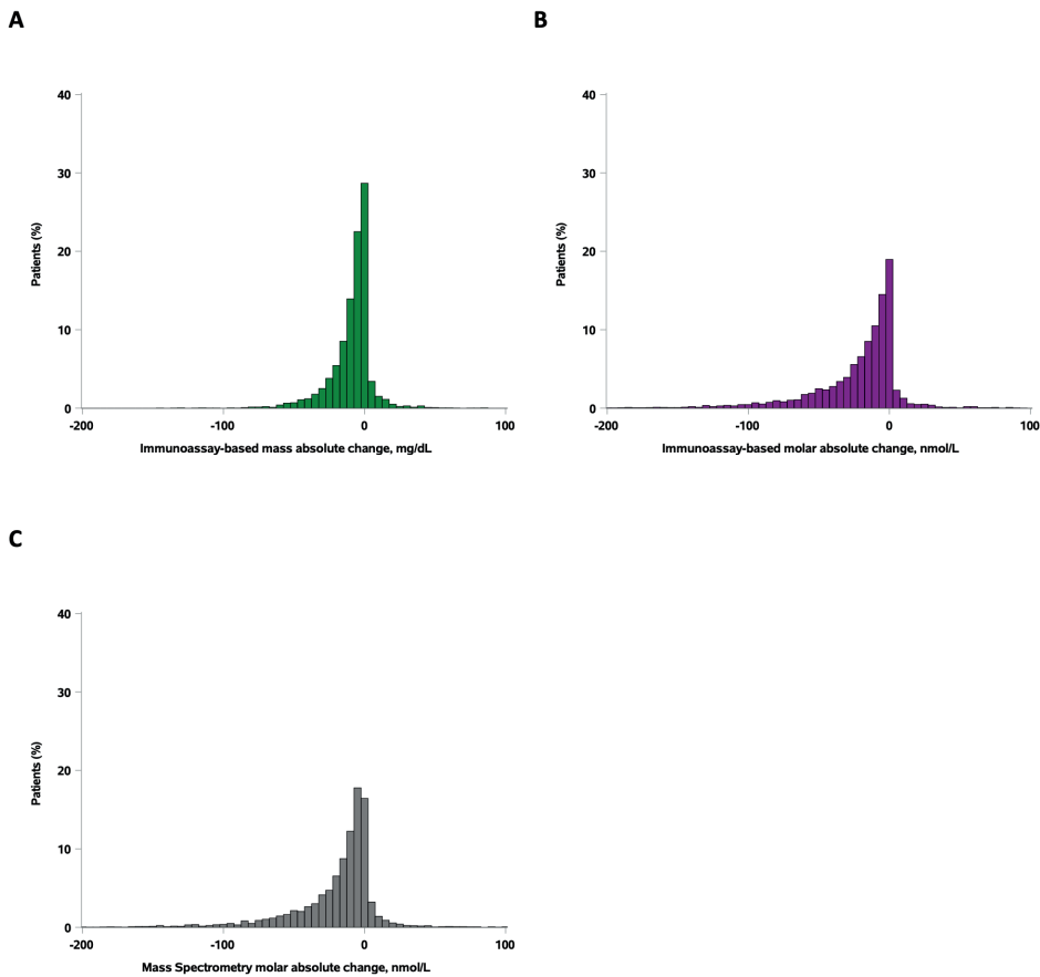
Figure S7: Histogram of absolute change in lipoprotein(a) concentrations from baseline to month 4 in the alirocumab group: (A) IA-mass; (B) IA-molar; and (C) MS. Median (IQR) absolute change in concentrations from baseline to month 4 within the alirocumab group were -5.1, (-13.4, 0) mg/dL for IA-mass, -11.9 (-32.0, -2.0) nmol/L for IA-molar, and -10.4 (-28.2, -2.7) nmol/L for MS. IA indicates immunoassay; MS, mass spectrometry.
