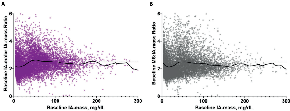
Figure S2: Scatterplots of baseline IA-mass lipoprotein(a) concentration by (A) the ratio of IA-molar to IA-mass lipoprotein(a) concentrations and (B) the ratio of MS to IA-mass lipoprotein(a) concentrations. Plots include 9990 patients who were above the lower limits of quantification on all three tests. Solid lines within plot are LOWESS curves utilizing 20 observations within the smoothing windows. Dashed horizontal lines designate a ratio of 2.5. IA indicates immunoassay; MS, mass spectrometry.
