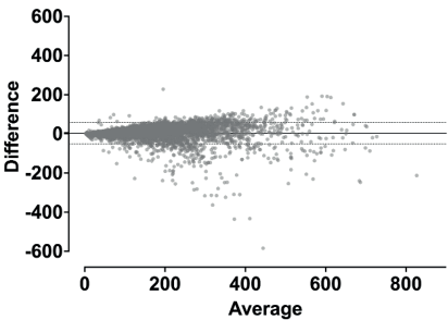
Figure S3: Bland-Altman analysis of baseline lipoprotein(a) IA-molar vs. MS concentrations. Overall bias was 3.8 nmol/L, with 95% limits of agreement of -50.7 to 58.3 nmol/L.
