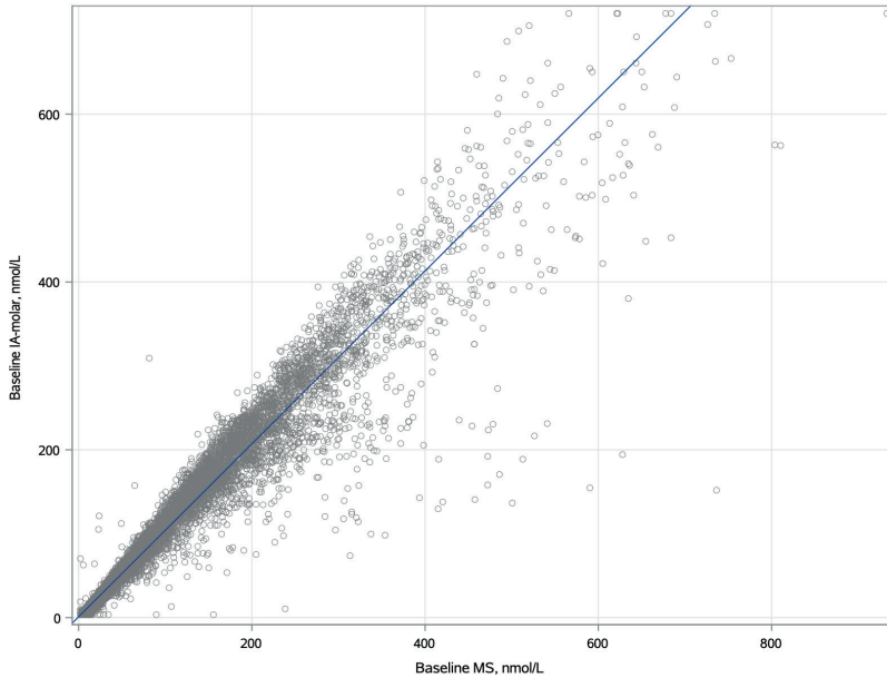
Figure S4: Deming regression analysis of baseline lipoprotein(a) IA-molar vs. MS concentrations. With MS specified as the predictor variable and IA-molar specified as the outcome, the estimated slope (95% confidence interval [CI]) is 1.03 (1.02, 1.04) and the estimated y-intercept is 1.07 (0.37, 1.78). The solid line within the plot reflects the estimated slope and y-intercept. Excluding participants below the lower limit of quantification on the MS test, the estimated slope (95% CI) is 1.03 (1.02, 1.04) and the estimated y-intercept is 1.01 (0.23, 1.79). Excluding participants below the lower limit of quantification on either test, the estimated slope (95% CI) is 1.03 (1.01, 1.04) and the estimated y-intercept is 1.72 (0.82, 2.63). IA indicates immunoassay; MS, mass spectrometry.
