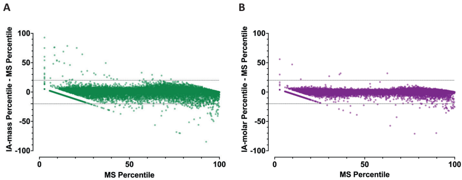
Figure 1: Baseline lipoprotein(a) MS concentration percentile vs difference in IA-mass and MS concentration percentiles and difference in IA-molar and MS concentration percentiles. Scatterplots of baseline lipoprotein(a) mass spectrometry (MS) concentration percentile vs difference in immunoassay-based mass test (IA-mass; A ) and MS concentration percentiles and MS concentration percentile vs difference in immunoassay-based molar test (IA-molar; B ) and MS concentration percentiles. IA-mass overestimated and underestimated concentration by \geq 20 ( \geq 10 ) percentiles compared with MS in 0.4% (3.9%) and 1.1% (8.0%) of patients, respectively. IA-molar overestimated and underestimated concentration by \geq 20 ( \geq 10 ) percentiles relative to MS in 0.1% (0.2%) and 0.4% (2.0%) of patients, respectively.
