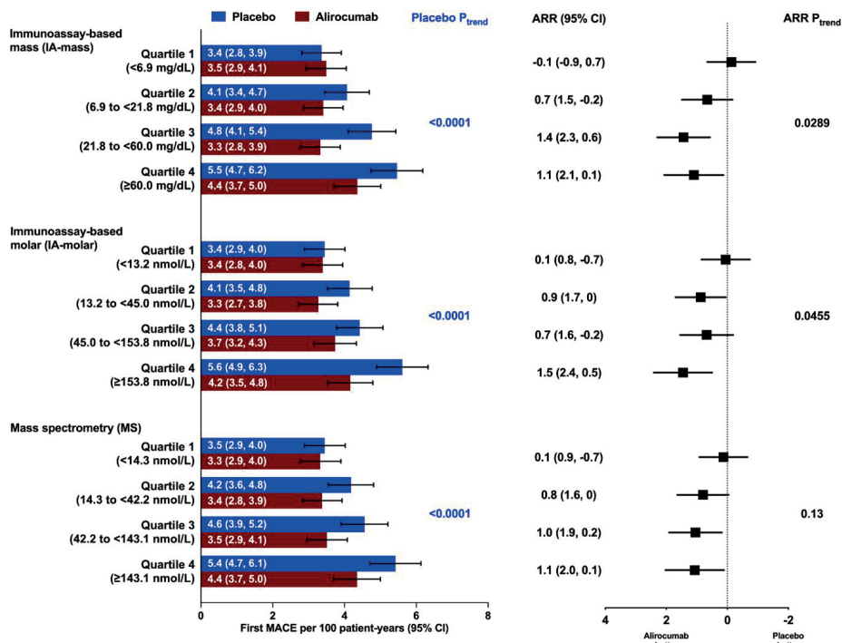
Figure 3: Rates of first MACE and absolute rate reductions with alirocumab stratified by baseline lipoprotein(a) IA-mass, IA-molar, and mass spectrometry concentration quartiles. Absolute risk reductions (ARRs) reflect number of first major adverse cardiovascular events (MACEs) avoided with alirocumab treatment per 100 patient-years. IA-mass indicates immunoassay-based mass test; and IA-molar, immunoassay-based molar test.
