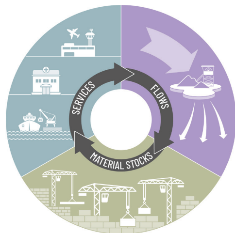
Figure 1. Dynamic feedback between stock, flows and services, creating a lock-in effect
