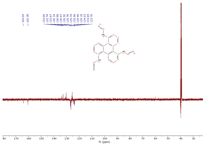
Figure 5.16: ^{13}\text{C} NMR spectrum of \text{N,N',N''} -(triphenylene-1,5,9-triyl)triformamide.
