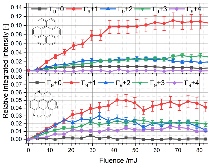
Figure 5.9: Comparison of the fragment ions formed in the dissociation of Cor \bullet^+ (top) and TAC \bullet^+ (bottom) in the mass range spanning m/z 108 to 112. The \Gamma_9 + 1 channels in both molecules are comprised of the initial \Gamma_9 + 1 signal as well as the \Gamma_{10} + 5 - 7 channels.
