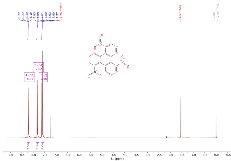
Figure 5.11: 1 H NMR spectrum of 1,5,9-trinitrotriphenylene.
