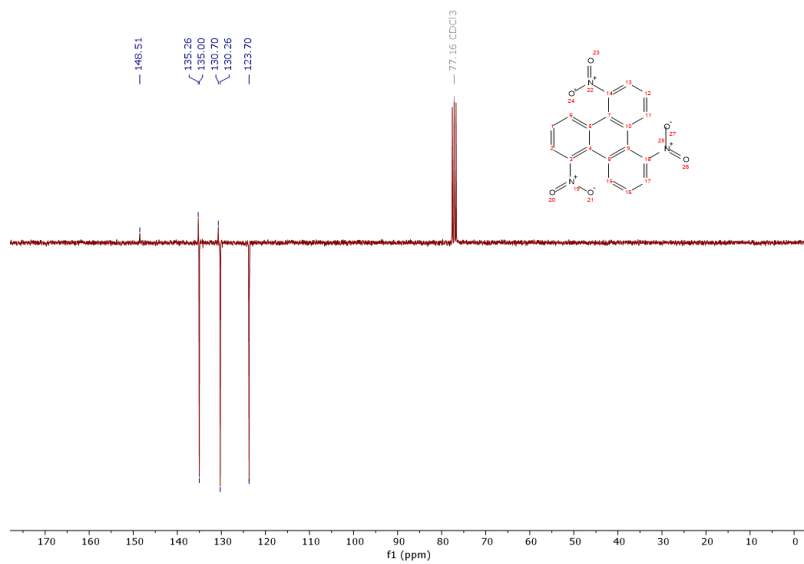
Figure 5.12: 13 C NMR spectrum of 1,5,9-trinitrotriphenylene.
