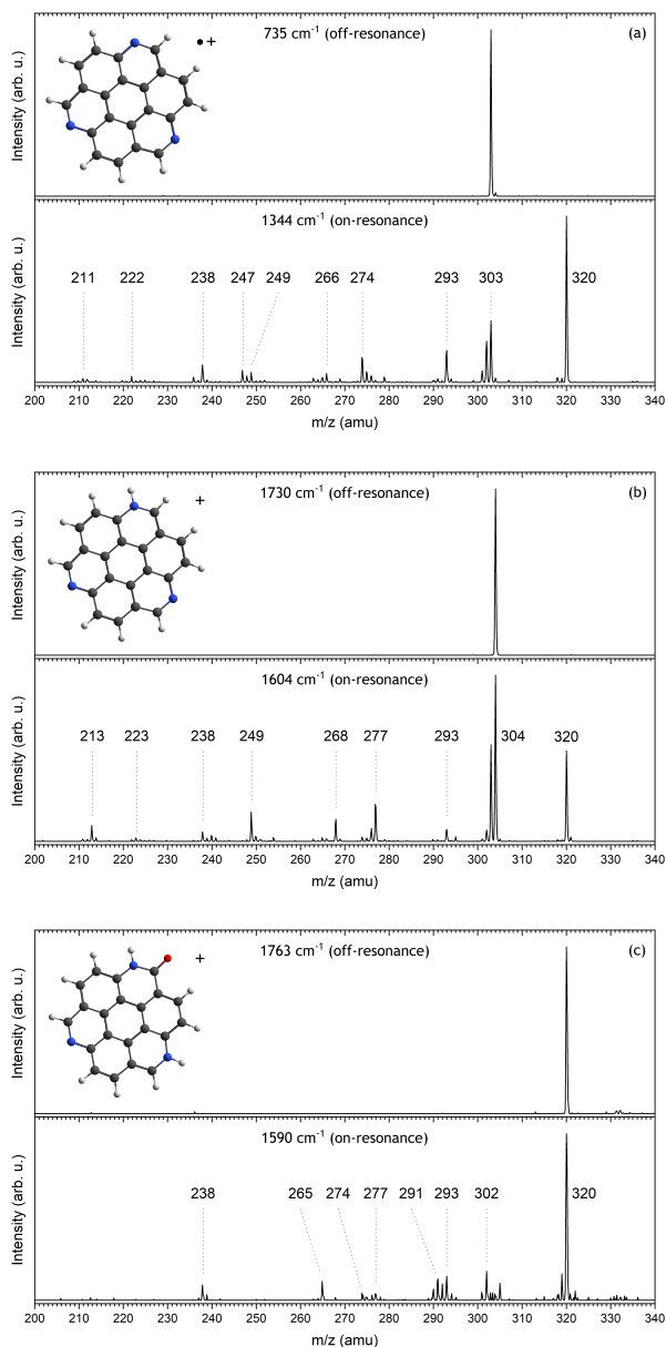
Figure 4.2: Mass spectra of isolated \text{TAC}^{\bullet+} (a), \text{TACH}^+ (b) and [\text{TAC}-\text{H}+\text{H}_2\text{O}]^+ (c) after exposure to off-resonance (top panel) and on-resonance (bottom panel) infrared radiation. The wavenumber of the IR radiation is depicted in each respective panel. The proposed geometry for the [\text{TAC}-\text{H}+\text{H}_2\text{O}]^+ species is discussed in section 4.3.4.
