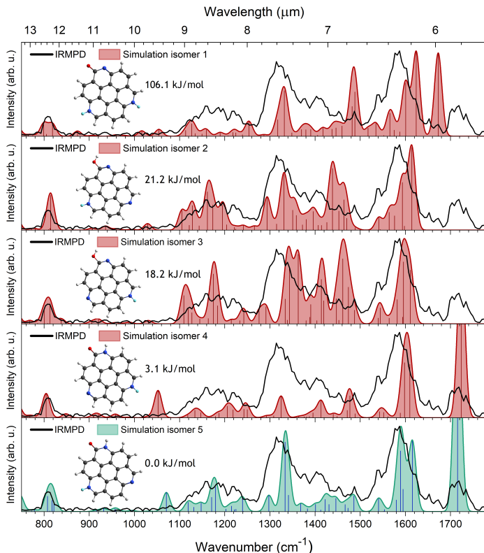
Figure 4.4: Experimental IRMPD spectrum (black) and simulated IR spectra of four different isomers of [\text{TAC-H}+\text{H}_2\text{O}]^+ . Also shown are the various structures of [\text{TAC-H}+\text{H}_2\text{O}]^+ isomers and their relative energies calculated using the B3LYP functional in combination with the 6-311++G(d,p) basis set. The hydrogen atoms that differ between the isomers are highlighted in cyan for clarity. The simulated spectrum in green indicates our tentative assignment that isomer 5 is likely the dominant isomer. The B3LYP/6-311++G(d,p) computed stick spectra are uniformly scaled with a factor of 0.9679. The calculated spectra are also convolved with a 20\text{ cm}^{-1} FWHM Gaussian function. All spectra are normalized with respect to their most intense peak in the wavenumber range 750\text{--}1650\text{ cm}^{-1} .
