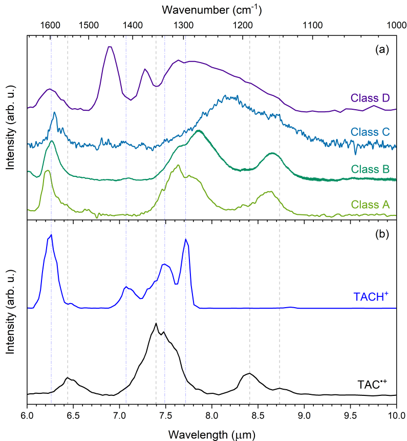
Figure 4.6: a) Mid-IR spectra of astronomical representative sources of type A (IRAS 23133+6050; olive), type B (HD 44179; green), type C (IRAS 13416-6243; blue), and type D (IRAS 05110-6616; purple). All are normalized to the maximum intensity of the 7–8 \mu\text{m} complex and with continuum subtracted. The type D spectrum was recorded using Spitzer/IRS (Werner et al. 2004; Houck et al. 2004) and the other classes are obtained from ISO/SWS (Kessler et al. 1996; de Graauw et al. 1996) observations, as calibrated by Sloan et al. (2003). b) Experimental IRMPD of \text{TAC}^{\bullet+} (black) and \text{TACH}^+ (blue). Both spectra are normalized with respect to their most intense peak. The vertical grey, dashed and blue, dot-dashed lines represent the peaks of the most clear features in the IRMPD spectra of \text{TAC}^{\bullet+} and \text{TACH}^+ , respectively.
