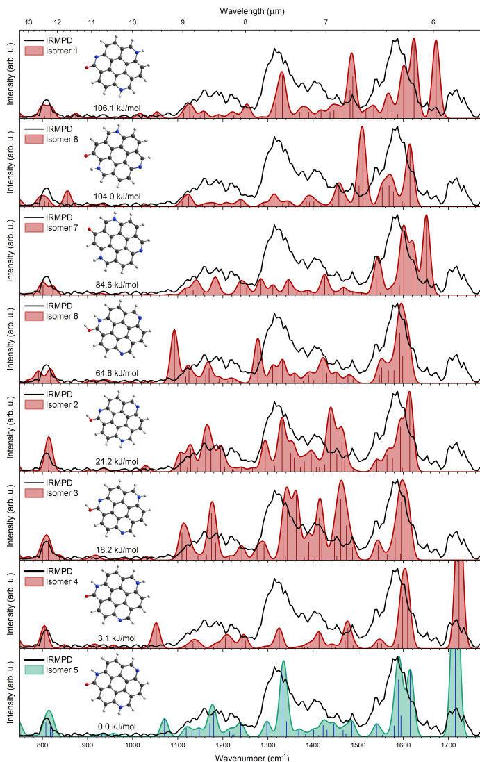
Figure 4.9: Experimental IRMPD spectrum (black) compared to simulated IR spectra of all considered isomers of [\text{TAC}-\text{H}+\text{H}_2\text{O}]^+ . Also shown are the structures of the various [\text{TAC}-\text{H}+\text{H}_2\text{O}]^+ isomers and their relative energies calculated using the B3LYP functional in combination with the 6-311++G(d,p) basis set. The simulated spectrum in green indicates our tentative assignment that isomer 5 is likely the dominant isomer. The B3LYP/6-311++G(d,p) computed stick spectra are uniformly scaled with a factor of 0.9679. The calculated spectra are also convolved with a 20\text{ cm}^{-1} FWHM Gaussian function to facilitate comparison with the experimental spectrum. All spectra are normalized with respect to their most intense peak in the 750\text{--}1650\text{ cm}^{-1} wavenumber range.
