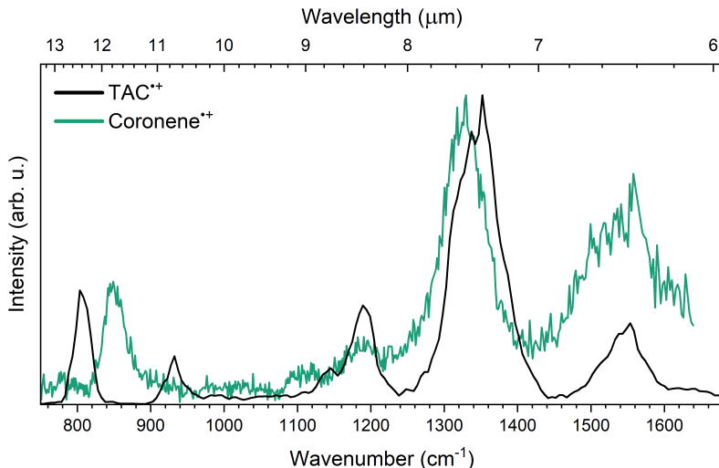
Figure 4.5: Experimental IRMPD of \text{TAC}^{\bullet+} (black) and coronene ^{\bullet+} (green). Both spectra are normalized with respect to their most intense peak. The IRMPD spectrum of coronene ^{\bullet+} is taken from Oomens et al. (2001)
