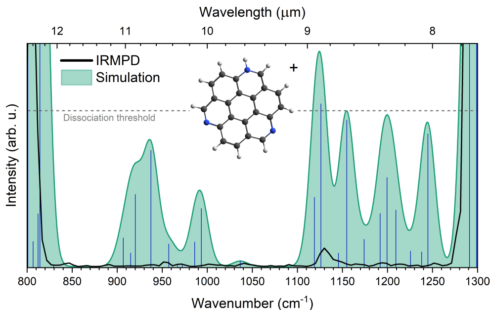
Figure 4.7: Experimental IRMPD (black) and simulated IR (blue vertical lines) spectra of \text{TACH}^+ . The B3LYP/6-311++G(d,p) computed spectrum (blue sticks) is uniformly scaled with a factor of 0.9679 and convolved with a 20 \text{cm}^{-1} FWHM Gaussian function (green shaded area). The horizontal grey, dotted line indicates an apparent cut-off. Exciting modes with a lower intensity than this line does not lift the energy of the molecule over the dissociation threshold.
