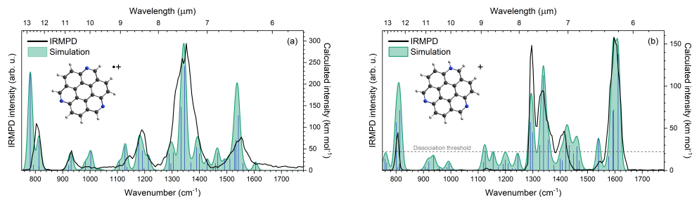
Figure 4.3: Experimental IRMPD (black) and simulated IR (blue vertical lines) spectra of TAC •+ (a) and TACH + (b). The B3LYP/6-311++G(d,p) computed spectrum (blue sticks) is uniformly scaled with a factor of 0.9679 and convolved with a 20 cm -1 FWHM Gaussian function (green shaded area). The IRMPD intensity is represented by the left axis and the intensity of the computed spectra by the right axis. All spectra are normalized to their most intense peak. The horizontal grey, dotted line in (b) indicates an apparent threshold of 21 km mol -1 . Exciting modes with an intensity below line does not allow the molecule to reach the dissociation threshold.
