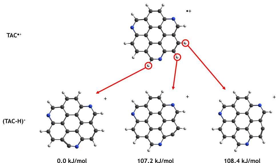
Figure 4.8: Geometries and relative energies of three different [\text{TAC-H}]^+ isomers calculated at B3LYP/6-311++G(d,p) level of theory. The circled hydrogen atoms on \text{TAC}^{\bullet+} depict the hydrogen that is removed and the arrows point toward the resulting isomer. The energies are depicted with respect to the lowest energetic isomer of [\text{TAC-H}]^+ .
