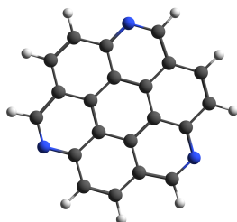
Figure 4.1: Molecular structure of cationic 1,5,9-triazacoronene ( \text{TAC}^{\bullet+} , \text{C}_{21}\text{H}_9\text{N}_3^{\bullet+} ).
