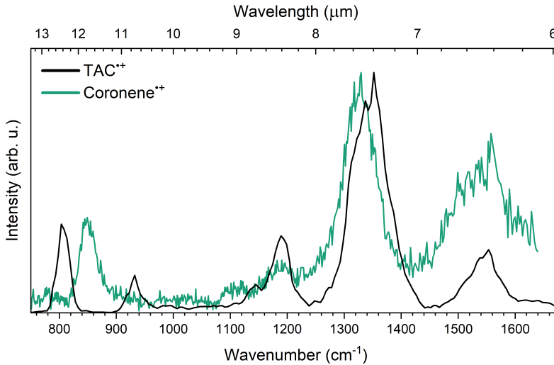
Figure 4.5: Experimental IRMPD of \text{TAC}^{\bullet+} (black) and coronene ^{\bullet+} (green). Both spectra are normalized with respect to their most intense peak. The IRMPD spectrum of coronene ^{\bullet+} is taken from Oomens et al. (2001)
