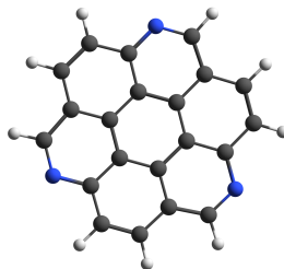
Figure 4.1: Molecular structure of cationic 1,5,9-triazacoronene ( \text{TAC}^{\bullet+} , \text{C}_{21}\text{H}_9\text{N}_3^{\bullet+} ).
