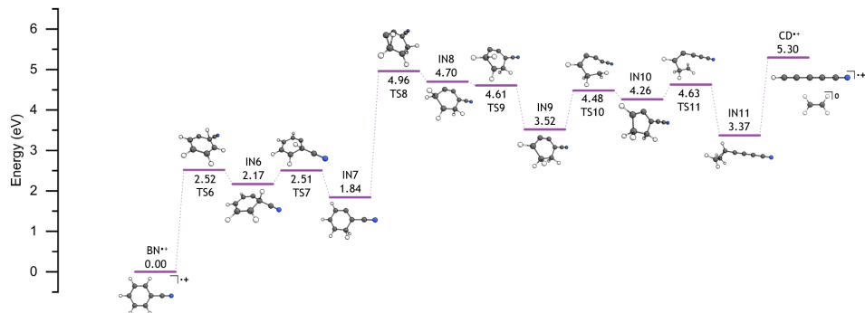
Figure 3.16: The benzonitrile ^{\bullet+} potential energy surface resulting in m/z 75 ( \text{HC}_5\text{N}^{\bullet+} ).
