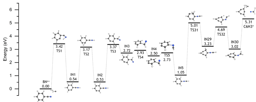
Figure 3.17: The benzonitrile •+ potential energy surface resulting in m/z 75 ( c\text{-C}_6\text{H}_3^+ ).
