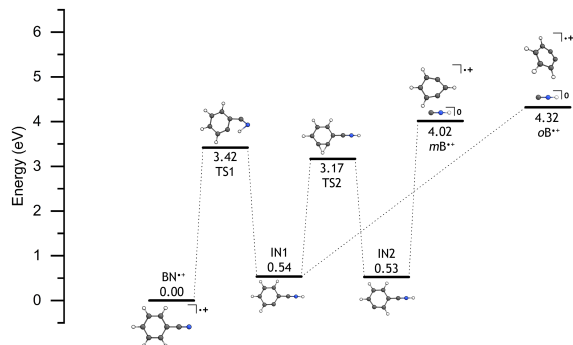
Figure 3.15: The benzonitrile ^{\bullet+} potential energy surface resulting in m/z 76 by loss of HNC. Both meta - and ortho -benzyne ^{\bullet+} are presented
