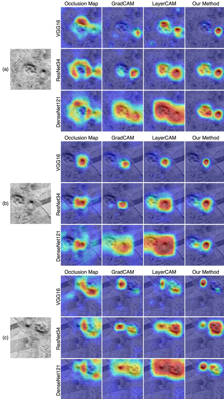
Figure 5.18: Different activations of Tell al-Shur ( 36.845^\circ N, 40.458^\circ E) with a complex morphology and a nearby conical site. Different augmentations of the same region are activated in different ways.
