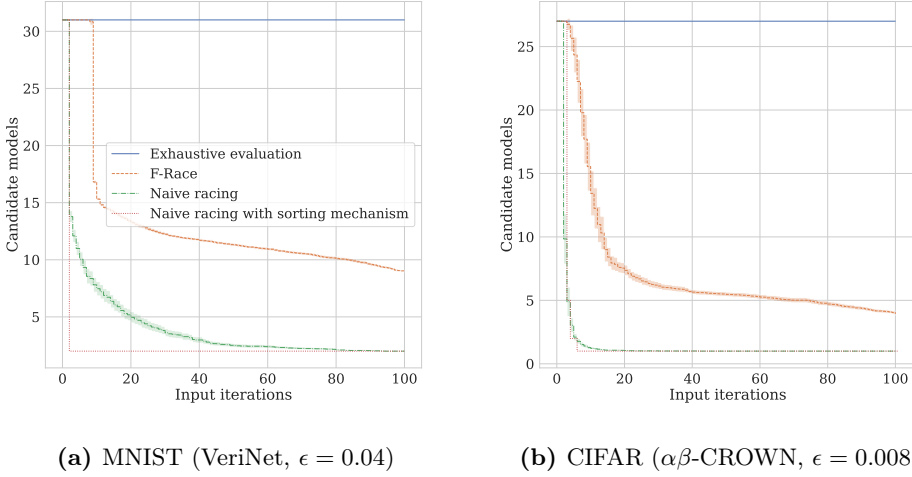
Figure 6.2: Number of candidate models as determined by each method after every input iteration. For the three methods that do not use the sorting mechanism, the line represents the average number of candidate models over 200 random input orders, each with different random seeds, along with the respective 95% confidence intervals. Clearly, naïve racing, coupled with our proposed sorting mechanism, reduces the number of candidates after substantially fewer input iterations than other methods. Notice that selection based on exhaustive evaluation does not eliminate models from the set of candidates, which, therefore, does not decrease in size.
