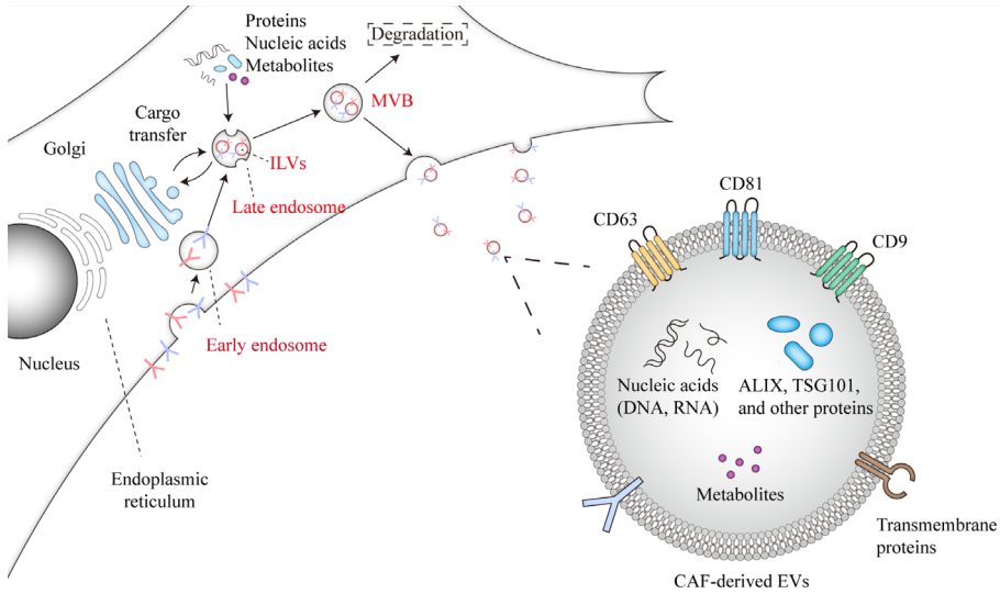
Figure 3. Schematic presentation of CAF-derived EVs. EVs can be released from the plasma membrane as ectosomes or from multivesicular bodies (MVBs) as exosomes. The biogenesis of exosomes mainly comprises three stages, which includes (i) the formation of early endosome by cytoplasmic membrane invagination, (ii) the formation of MVBs containing cargos-enriched ILVs, and (iii) the release of ILVs as exosomes after the fusion of MVBs with the plasma membrane.
