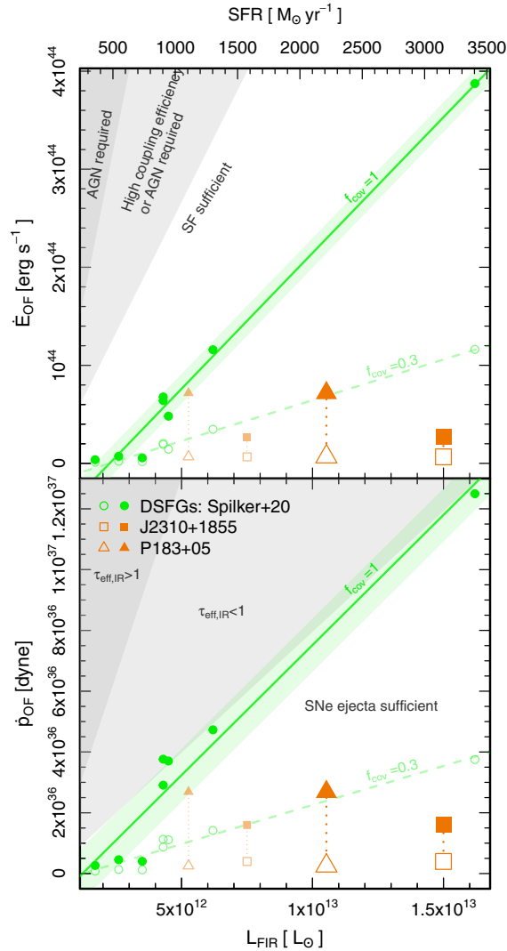
Figure 1. From Butler et al. (2023a) : Comparing Molecular outflows from high- z unobscured QSOs with high- z DSFGs ( Spilker et al. 2020b ). The kinetic energy flux (top) and momentum flux (bottom) as a function of FIR luminosity and SFR. The unobscured QSOs (orange) do not require input from an AGN to drive their molecular outflows and in fact, appear to be suppressed after the blow-out phase compared to the DSFGs. This implies that the central AGN is not the dominant driving mechanism of outflows in the unobscured QSOs.
