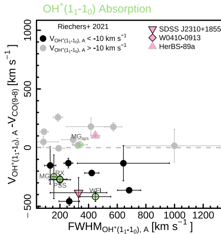
Figure 2. Adapted from Butler et al. (2023b) : Comparing predominantly atomic gas outflows from high- z unobscured QSOs with high- z DSFGs ( Riechers et al. 2021 ). The line width versus outflow velocity of the predominantly atomic gas: the outflows driven from the QSO sample (green) are not boosted with respect to the DSFG. This implies that the central AGN is not the dominant driving mechanism of outflows in the unobscured QSOs.
