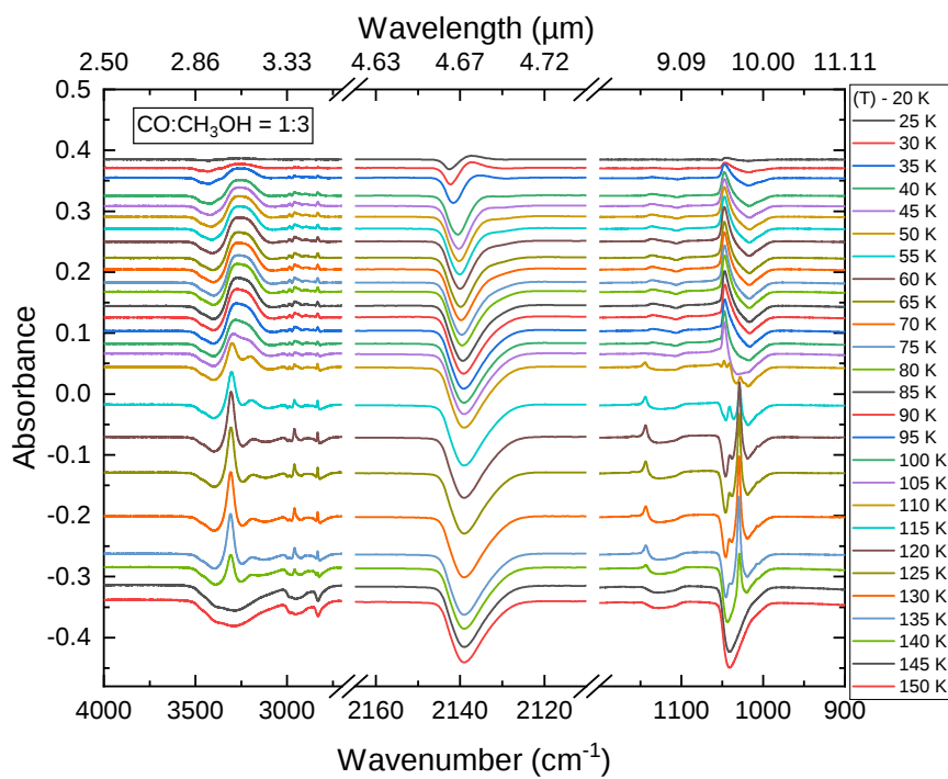
Figure 3.11: Control IR difference spectra of the \text{CO}:\text{CH}_3\text{OH} = 1:3 ice mixture acquired during TPD.
