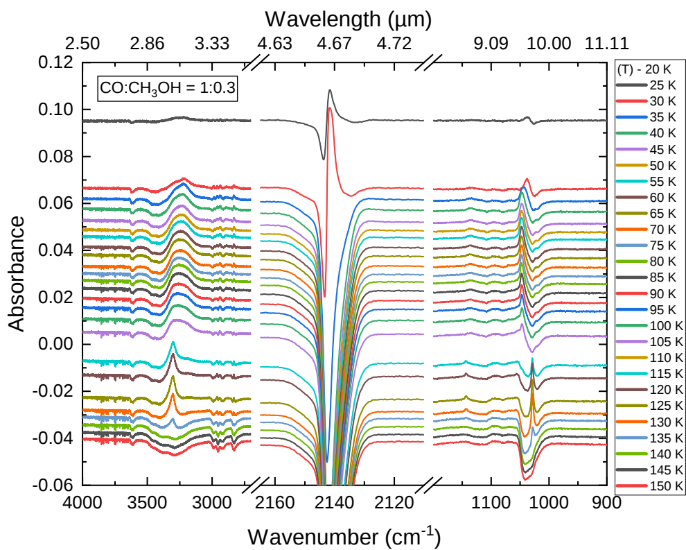
Figure 3.10: Control IR difference spectra of the \text{CO}:\text{CH}_3\text{OH} = 1:0.3 ice mixture acquired during TPD.
