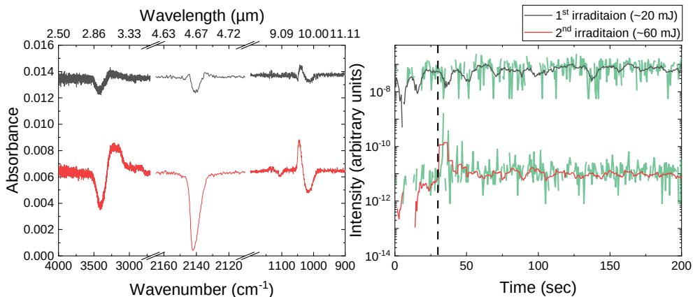
Figure 3.7: IR and QMS data obtained for two successive 9.62\ \mu\text{m} FEL exposures of the methanol-rich ice performed at the same substrate position (i.e., without moving the translation stage) and at 20 K. The first (black) irradiation was attenuated to a power of \sim 20\ \text{mJ} , whereas the second (red) is performed at the full attainable power of \sim 60\ \text{mJ} . Left panel: Difference of the spectra acquired before and after the irradiations. The spectra are offset for clarity. Right panel: Superposition of the QMS data for the mass signal of CO ( m/z = 28 ) measured concomitantly to the IR spectra during the FEL exposures (green lines) and their corresponding smoothed signal (black and red lines). The dashed line indicates the beginning of the irradiations.
