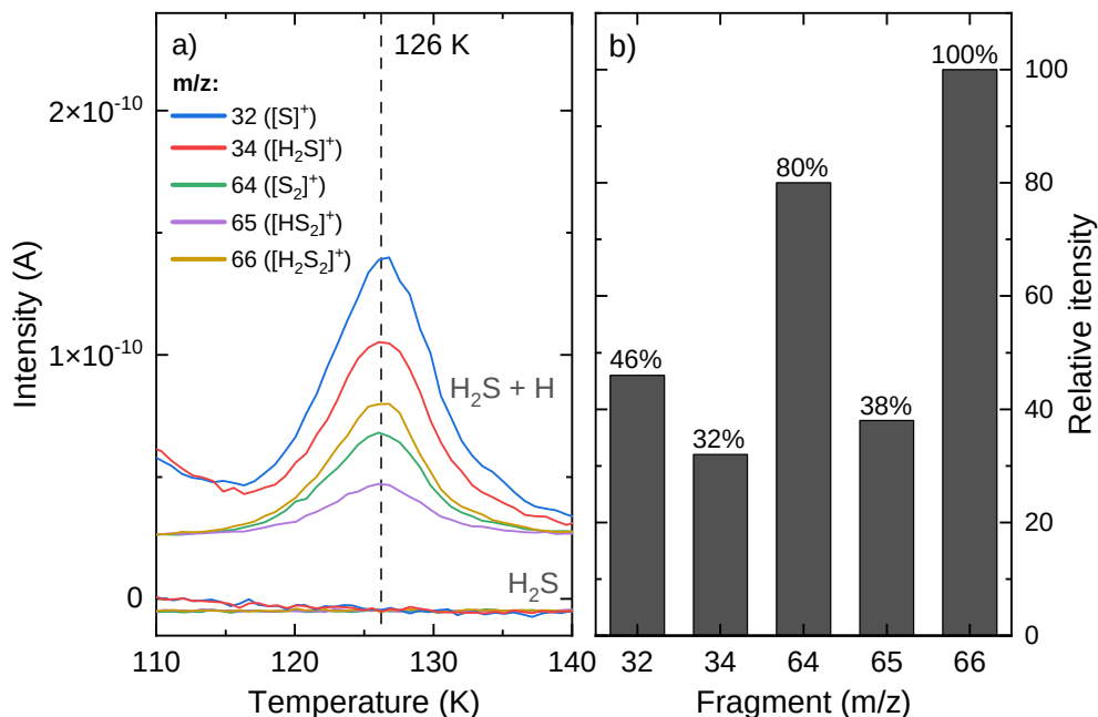
Figure 4.3: TPD-QMS results for the detections of H_2S_2 . Panel a): TPD-QMS spectra of m/z = 32 (blue), 34 (red), 64 (green), 65 (purple), and 66 (yellow) after deposition of a pure H_2S ice and codeposition of H_2S + H with analogous experimental conditions. Spectra are offset for clarity and shown in the temperature range relevant to H_2S_2 thermal desorption. Panel b): Mass fragmentation pattern of H_2S_2 generated by 70 eV electron ionization as measured in this work.
