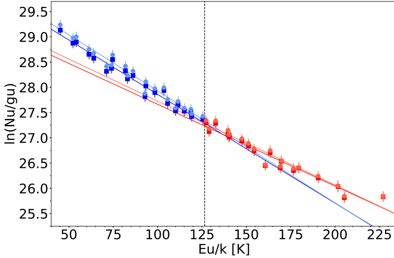
Figure 9.8: Rotational diagram of the \text{CH}_3\text{CCH} lines for a source size of 10'' . The points were divided into two subsets indicated by the dashed line. The points pertaining to the low- and high-energy subsets are shown in blue and red, respectively. Least squares fits to the points within each subset are shown. Circles and squares correspond to the lines with and without opacity corrections, respectively.
