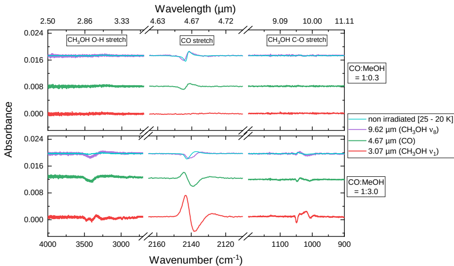
Figure 3.6: Difference spectra obtained before and after five minutes of IR-FEL irradiation on ice mixtures of CO and \text{CH}_3\text{OH} at 20 K. Upper panel: Mixture ratio of \text{CO}:\text{CH}_3\text{OH} = 1:0.3 . Lower panel: Mixture ratio of \text{CO}:\text{CH}_3\text{OH} = 1:3.0 . The control TPD difference spectra between 25 K and 20 K are also shown in cyan. The irradiation spectra are offset for clarity.
