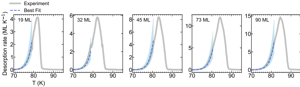
Figure 5.2: TPD curves of the multilayer \text{H}_2\text{S} ice experiments. The experimental data is shown in gray, while the zeroth-order Polanyi-Wigner models are shown with the dashed blue curve. The shaded blue region indicates the 1\sigma uncertainty.
