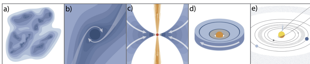
Figure 1: Stages of star and planet formation in Sun-like systems. (a) Dense pockets exist in inhomogeneous clouds of gas and dust. (b and c) These pockets collapse under gravity to form a young star. (d) The surrounding cloud material is dispersed, leaving a young star with a disk where planets can form. (e) Eventually, the disk disappears and gives rise to a planetary system. Adapted from Öberg & Bergin (2021).
