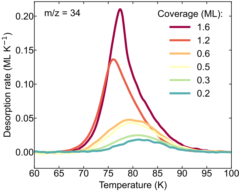
Figure 5.3: TPD curves of the low-coverage \text{H}_2\text{S} ice experiments deposited on top of a cASW substrate. The transition from zeroth-order to pure first-order sublimation behavior is seen for coverages < 1.2 ML. The experimental data is smoothed for clarity.
