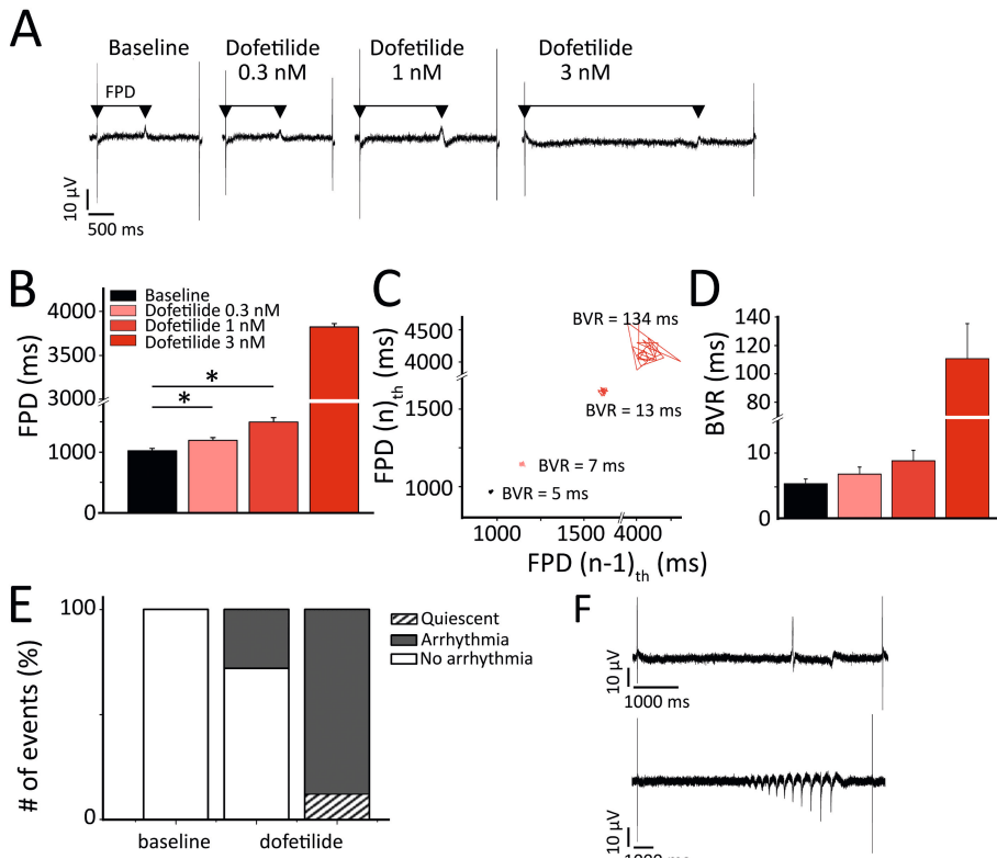
Figure 6. Repolarization instability and arrhythmia in MEAs upon I_{Kr} block. (A) Representative field potentials, at escalating dofetilide concentrations (0.3, 1, 3 nmol/L). The arrows indicate the FPD. (B) Average values of FPD for each dofetilide concentration (n = 4 per condition). (C) Poincaré plot depicting the FPD BVR at escalating dofetilide concentrations for a selected electrode. (D) Average values of FPD BVR in MEAs (n=4). (E) Arrhythmia inducibility as percentage of total events, at baseline and during dofetilide 3 and 10 nmol/L (n=8 per condition). (F) Representative examples of two types of arrhythmia [single abnormal impulse (above) and burst (below)] triggered by dofetilide.
