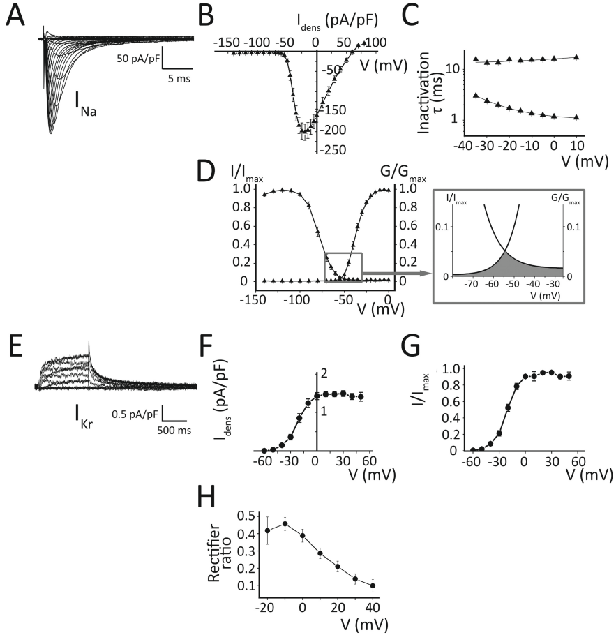
Figure 2. Ion currents in Pluricyte® CMs. (A) Voltage-dependent I_{Na} activation; representative family of traces. (B) I_{Na} -density I - V relationship ( n = 19 ). (C) Kinetics of voltage-dependent steady-state inactivation, obtained by a double exponential fit. (D) Steady-state activation and inactivation, with conductance and current normalized to their maximum values. Inset shows the 'window-current', as the area under the crossing between the steady-state activation and inactivation curves. (E) Voltage-dependent I_{Kr} activation. (F) I_{Kr} -density I - V relationship ( n = 18 ). (G) Steady-state activation of I_{Kr} ; current normalized to maximum value. (H) Rectifier ratio, correlating the conductance of the depolarizing step with the I_{Kr} -tail conductance.
