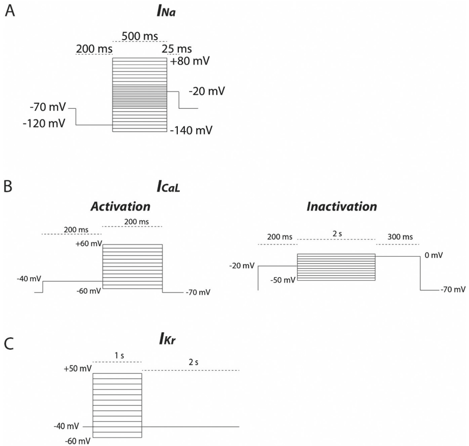
Figure S1: Protocols used for the voltage-clamp experiments, for I_{Na} , I_{CaL} and I_{Kr} .
