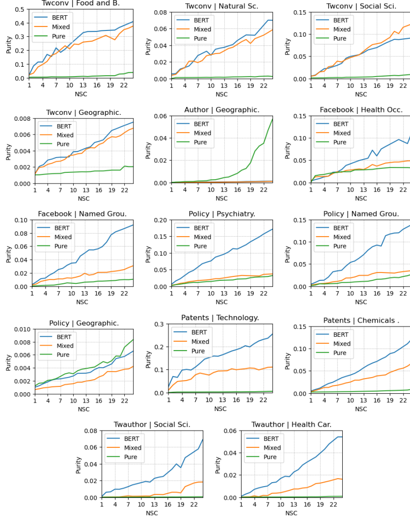
Figure 3: Examples of Purity of several topic categories for different networks. All profiles are for Size bin 161-320 and Coverage 0.50. To interpret these plots, it is important to keep in mind that each profile represents the average Purity and NSC across all topics in the topic category and Size bin, based on multiple clustering solutions. One way to interpret each curve is as if it were the Purity profile of a single, imaginary topic that combines all the topics in the category, including both the high- and low-performing ones. This topic would contain 240 documents (the average size of the bin), with each NSC value in the curve including 120 topic documents (due to Coverage 0.50). Purity values should not be compared across different sources, as some networks are substantially smaller, reducing clustering quality due to lack of information and making such comparisons unfair.
