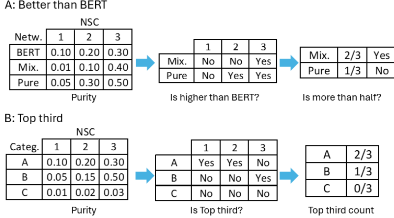
Figure 2: Diagram on the representation of results. A: How to calculate from topic Purity profiles if a topic has higher clustering effectiveness than BERT in the Pure or the Mixed network. In this example, a topic has higher Purity than BERT for the Mixed network, but not so for the Pure network. B: How to calculate from topic category Purity profiles the number of NSC that a topic category is in the top third Purity of a network. In this example, the topic categories A, B and C achieve a top third count of 0.7, 0.3 and 0, respectively.
