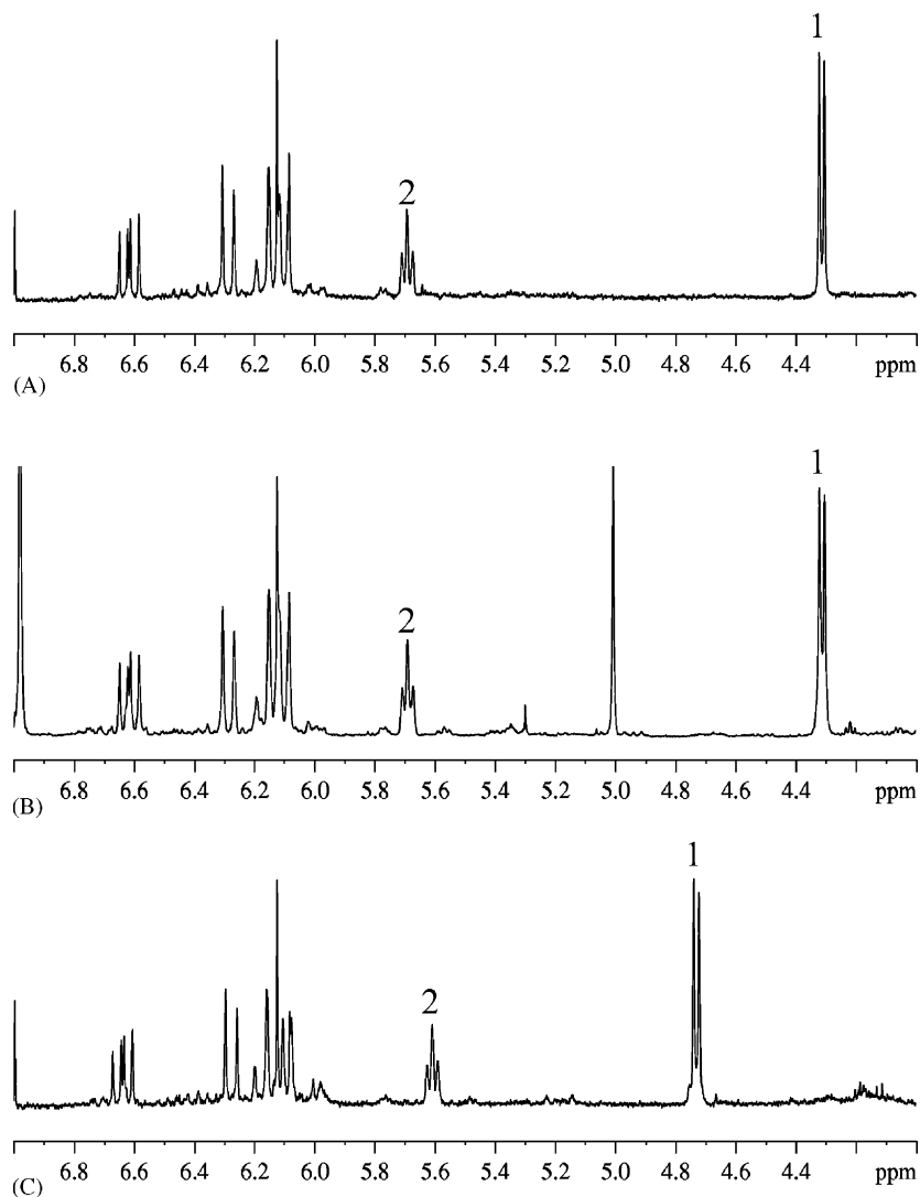
Fig. 2. The 400 MHz 1 H-NMR spectrum of the reference compounds: (A) retinol, (B) retinol palmitate after saponification, and (C) retinol palmitate in the range of \delta 4.0–7.0 in CDCl 3 . (1) H-15; (2) H-14.
