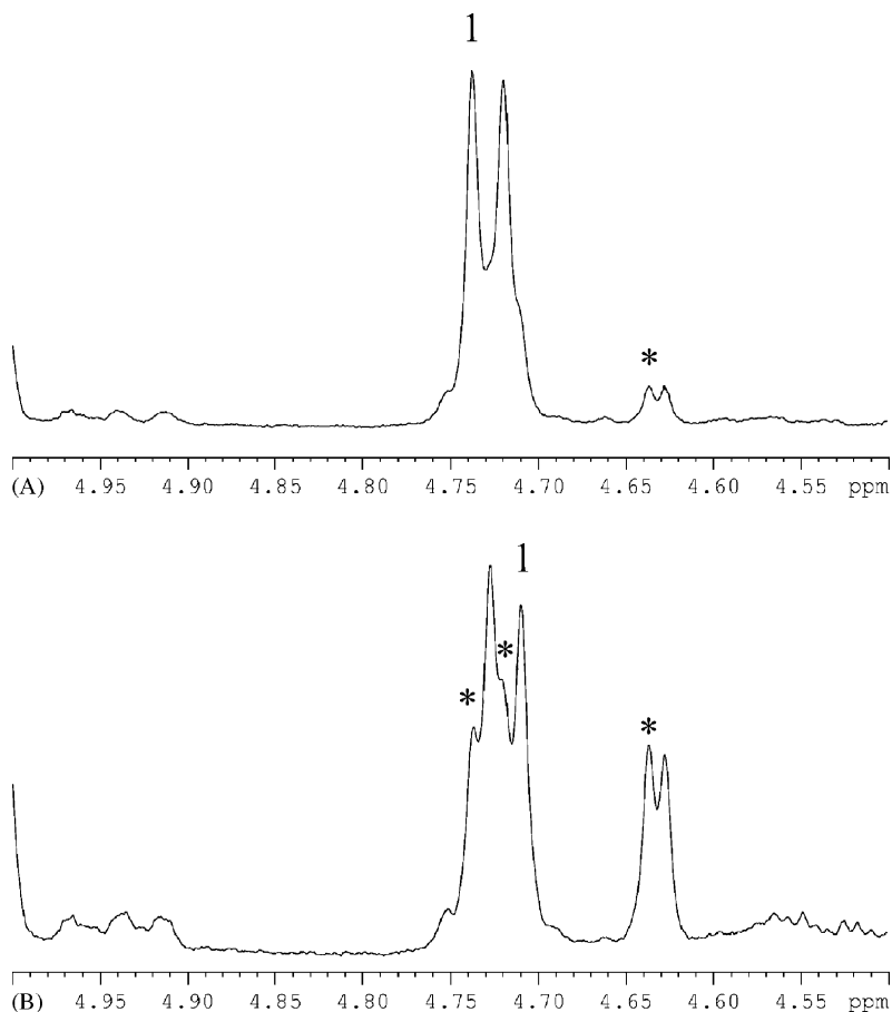
Fig. 5. The 400 MHz ^1\text{H} -NMR spectrum of Essential Vitamine A ® : (A) after 10 min and (B) 24 h in the light in the range of \delta 4.5–5.0 ( \text{CDCl}_3 ). (1) H-15; (*) possible isomerised peaks of retinol palmitate.
