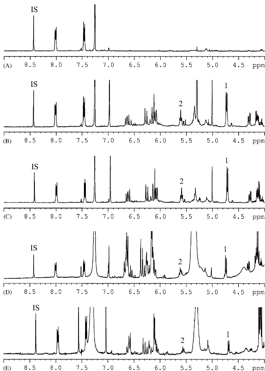
Fig. 4. The 400 MHz ^1\text{H} -NMR spectrum of: (A) blank sample, (B) Essential Vitamine A ® , (C) Essential Vitamine A&D ® , (D) Essential Organics Megavites ® , and (E) Essential Organics All Sports ® in the range of \delta 4.0–7.0 ( \text{CDCl}_3 ). (1) H-15; (2) H-14; IS: H-9 and H-10 of anthracene (internal standard).
