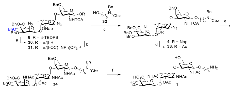
Scheme 4: Deprotection of the trisaccharide to form target 1 . Reaction conditions: a) TBAF, AcOH, THF, 0 °C to rt, 81%, b) ClC(=NPh)CF 3 , K 2 CO 3 , acetone, 92%, c) TBSOTf, DCM/MeCN, -50 °C, 73%, d) i) DDQ, DCM/H 2 O, ii) Ac 2 O, DMAP, pyridine, 89 % over two steps, e) zinc, AcOH, Ac 2 O, THF, 50 °C, 18%, f) Pd(OH) 2 /C, AcOH, H 2 , t -BuOH/H 2 O, 56%.
