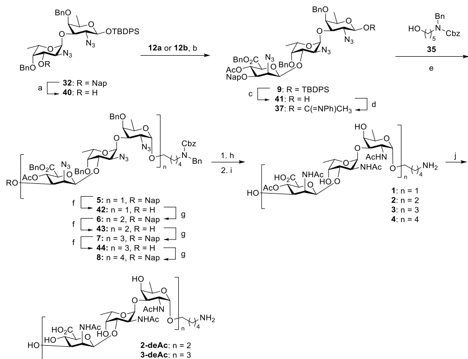
Scheme 3: Synthesis of the target oligosaccharides 1 , 2 , 3 and 4 . Reaction conditions: a) DDQ, DCM/H 2 O, 86%, b) TfOH, DCM, -78 to -10 °C, 66%, \alpha/\beta = 14:86, c) TBAF, AcOH, THF, 0 °C to rt °C, 84%, d) ClC(=NPh)CF 3 , K 2 CO 3 , acetone, 93%, e) TMSI, Ph 3 P=O, DCM/Et 2 O, 83%, \alpha/\beta = 75:25, f) DDQ, DCM/H 2 O, 42 =80%, 43 =54%, 44 =57%, g) 37 , TBSOTf, DCM, 6 =87%, 7 =77%, 8 =68%, h) zinc, AcOH, Ac 2 O, THF, 50 °C, i) Pd(OH) 2 /C, AcOH, H 2 , t -BuOH/H 2 O, yield over two steps 1 =45%, 2 =37%, 3 =57%, 4 =33%, j) 1 M NaOH in H 2 O, 2-deAc =41%, 3-deAc =46%.
