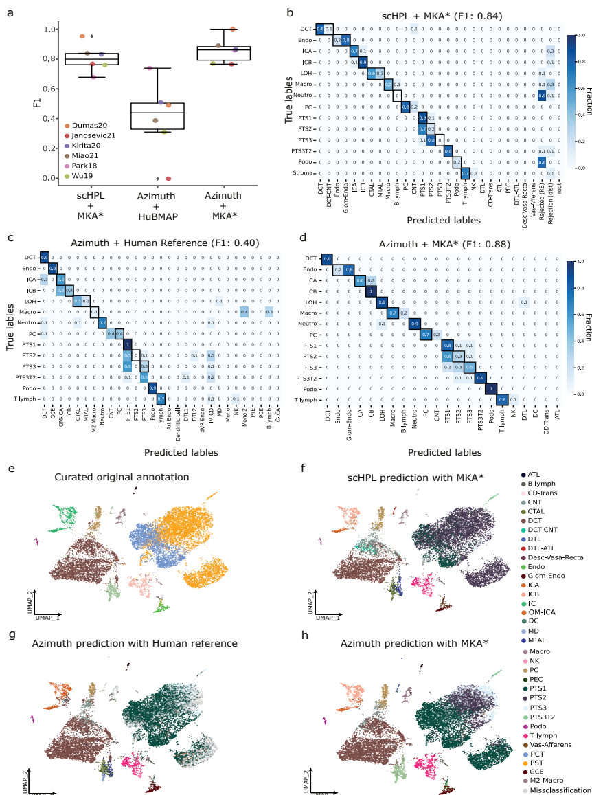
Figure 2.4: Evaluation of the schHPL classifier. a Boxplot of median F1 scores (y-axis) computed over six folds in three different scenarios (x-axis). From left to right, schHPL trained with MKA*, Azimuth's label transfer using the HubMAP reference available 104 , and Azimuth's label transfer using MKA* as reference. Each dot corresponds to the median F1 score computed across cell populations for a given training and validation set (i.e., MKA* and each of the annotated datasets in MKA, respectively). b-d Confusion matrices normalized by class support size, computed using the predicted annotations by schHPL and our Atlas reference ( b ), the transferred labels from Azimuth's human kidney reference 103 ( c ), or the transferred labels from Azimuth using our reference ( d ). Higher values indicate higher agreement between predicted and true cell labels. e-h UMAP plot of the Miao21 dataset coloured by the original cell types (after manual re-annotation) ( e ), by the predicted cell types from the learned classification tree ( f ), by the transferred cell types from the Azimuth human reference ( g ), and by the transferred labels using Azimuth with our Atlas reference ( h ).
