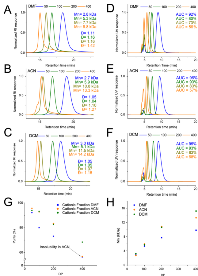
Figure 1. (A–C) DMF-SEC chromatograms of pSar with different [M]/[I] synthesized in DMF, ACN, and DCM, respectively. (D–F) CEC of pSar with different [M]/[I] synthesized in DMF, ACN, and DCM, respectively. (G) Purity as a function of DP of ROPs in different solvents as assessed by CEC. (H) M_n as a function of DP for ROPs in DMF, ACN, and DCM, respectively.
