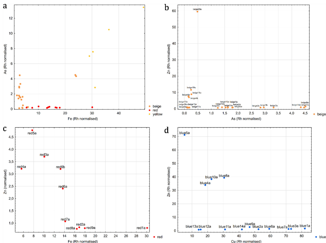
Fig. 6 Rh normalised scatter plot of net peak intensities of a beige, red and yellow pigments showing enrichments in both Fe and As for the yellow pigments, as well as enrichment in As for the beige layers and Fe for the red layers; b the beige areas showing either Zn or As enrichments; c Fe-rich and Zn-rich red pigments d ; Zn and Cu for the blue pigments, clearly delineating Zn enriched measurements from purely copper based pigments
