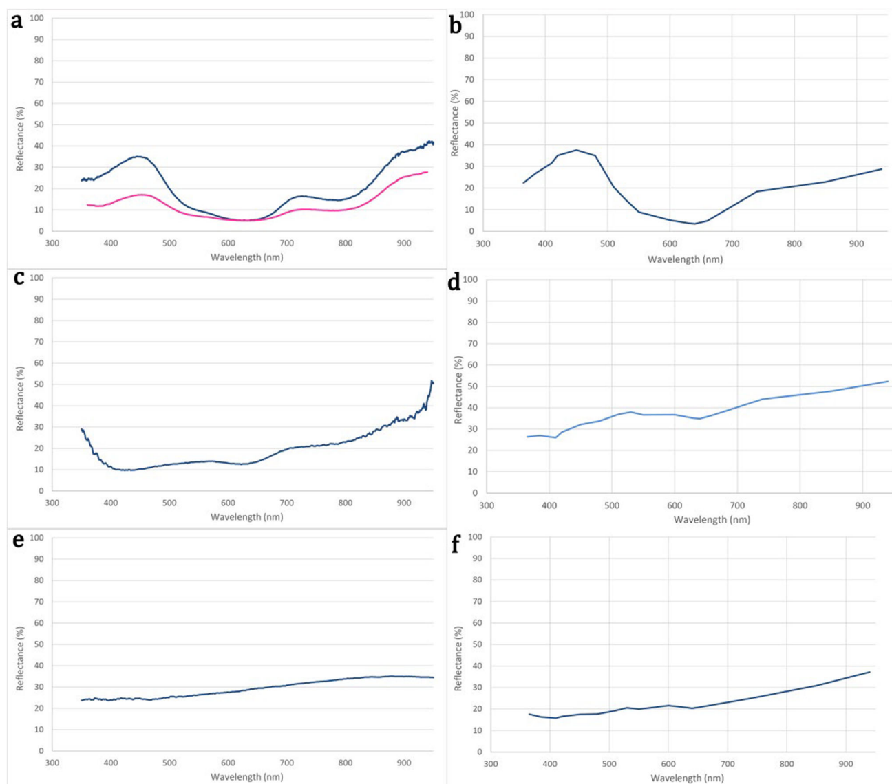
Fig. 4 Comparison of FORS and NBMSI spectral curve measurement on blue pigments. a FORS measurements on modern Egyptian blue samples, blue graph: on Pigment Checker v.5 with the KU Leuven device; pink graph: plot by CHSOS as included in the Gorgias database; b spectral curve measurement with NBMSI cube on modern Egyptian blue sample on Pigment Checker v5; c FORS measurement blue02 on pale blue pigment; d NBMSI measurement blue005 on pale blue pigment; e FORS measurement blue01 on darker blue pigment; f NBMSI measurement blue006 on darker blue pigment
