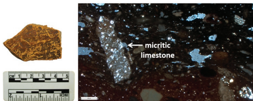
Figure 65: S77 - SW from Ambelikou-Agios Georghios, assigned to Fabric III (photomicrographs taken under XP x2,5)
