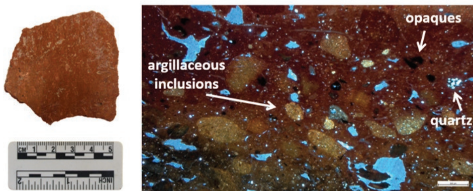
Figure 57: S47 – RB/B from Kissonerga-Mosphilia , assigned to Fabric I (photomicrograph taken under XP x2,5)
