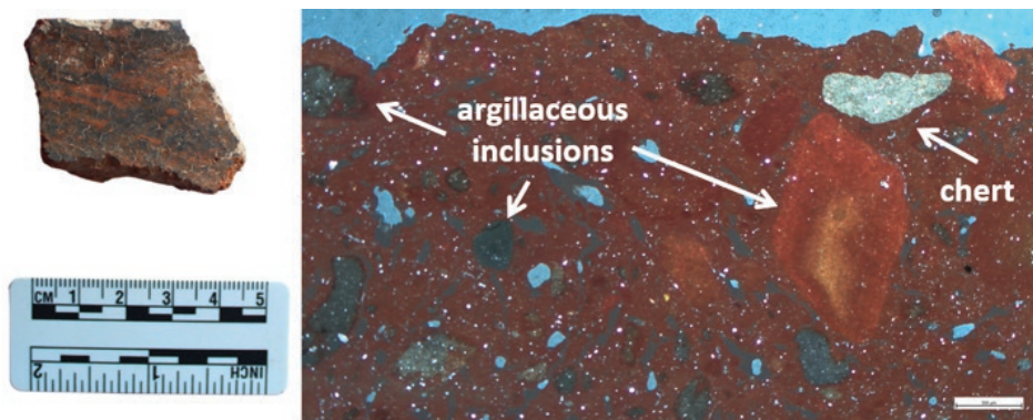
Figure 56: S31 – RB/B from Chlorakas-Palloures , assigned to Fabric I (photomicrograph taken under XP x2,5)
