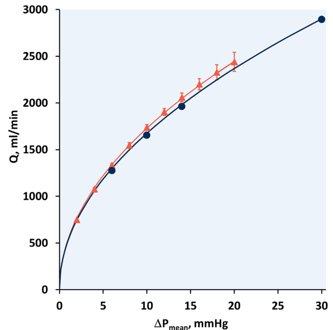
Figure 2 Computational flow dynamics (CFD) and in vitro bench measurement of shunt device flow/pressure relationship. ● represents data from CFD simulations in blood and ▲ are bench measurements in saline. Error bars are standard deviations. Curved lines are respective fits to model haemodynamic equation (1) with R^2 > 0.99 for each fit. \Delta P , mean pressure gradient; Q , flow.
