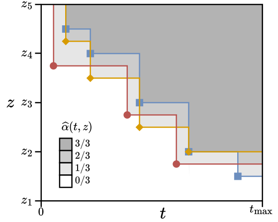
Figure 1. Visualization of the EAF corresponding to three runs (red circles, orange diamonds, and blue squares) of an hypothetical single-objective optimizer. For each run, we record as a point, the runtime t (x-axis) at which a new best-so-far objective function value z (y-axis) was found (assuming minimization). The value of the EAF \hat{\alpha} at point (t, z) is given by the shade of gray specified in the legend. We mark 5 quality targets in the y-axis \{z_1, z_2, \dots, z_5\} for computing the target-based ECDF in Figure 2.
