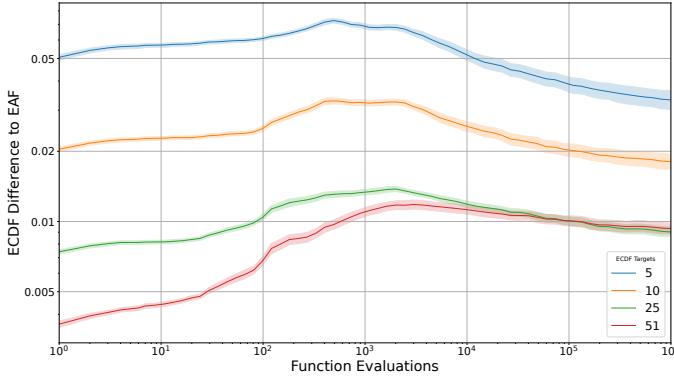
Figure 8. Mean and standard deviation of differences in target-based ECDFs with different numbers of targets relative to the EAF-based ECDF. Each individual ECDF value is an aggregation of the 24 10-dimensional BBOB problems for one algorithm. These are aggregated over all 211 processed algorithms from COCO's repository. Both axes are in logarithmic scale.
