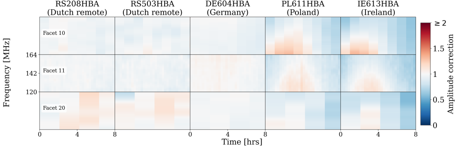
Figure 4.10: Merged amplitude calibration solution plots corresponding to the different facets (rows) and different stations, given by their station IDs (columns). The facets have the DD solutions from their corresponding calibrator, as depicted in Figure 4.14.
