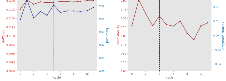
Figure 4.31: Self-calibration and solution stabilities for the source in the upper panel of Figure 4.30. The interpretation of these figures is discussed in the captions of Figures 4.12 and 4.13. It is important to note that this source did not have amplitude corrections, as according to the auto settings from facetselfcal , this source was not sufficiently bright enough to trigger scalarcomplexgain corrections.
