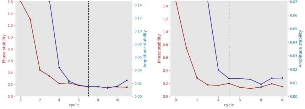
Figure 4.13: Self-calibration solution stability for two different sources (corresponding to the sources from Figure 4.12). The red line displays the circular standard deviation of the phase solution difference between the current and previous self-calibration cycle for each time and frequency value for each station. The blue line gives the standard deviation of the amplitude ratio of each time and frequency value for each station between the current and previous self-calibration cycle. We note that amplitude solves are only optionally triggered from cycle 3 onward, when the S/N is deemed sufficient by metrics from facetselfcal . The black dashed line corresponds to the selected calibration cycle, based on a combined assessment of the solution and image stability.
