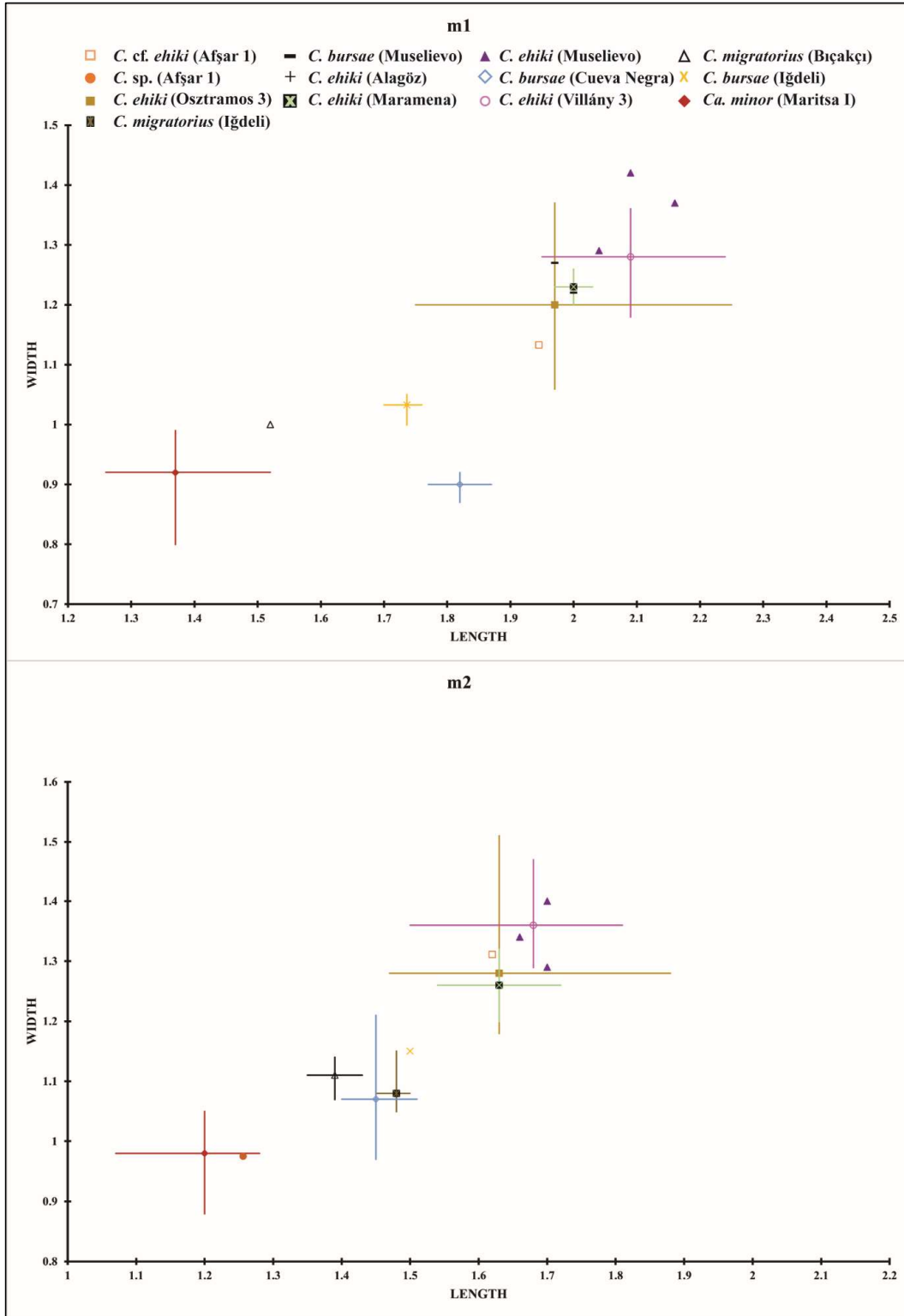
Figure 18. L/W scatter plot of the m1 and m2 from Cricetulus cf. ehiki and Cricetulus sp. from Afşar 1; C. ehiki from Osztramos 3 (MN 17), Villány 3 (MN 17), Alagöz (MN 14), Maramena (MN 13), Muselievo (MN 15) (Daxner-Höck, 1992; Hír, 1993a; Popov, 2004; Čermák et al., 2019); C. migratorius from İğdeli (MN 14) and Bıçakçı (MN 17) (Suata-Alpaslan et al., 2010; Hoek Ostende et al., 2015); C. bursae from Cueva Negra (late Early Pleistocene, İğdeli and Muselievo) (Popov, 2004; Suata-Alpaslan et al., 2010; Hoek Ostende et al., 2015); Calomyscus minor , from Maritsa I (MN 13) (De Bruijn et al., 1970). Measurements were made in mm.
