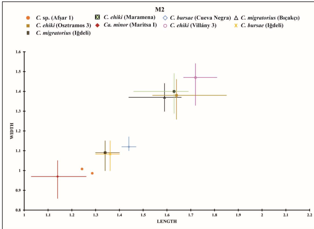
Figure 17. L/W scatter plot of the M2 from Cricetulus sp. from Afşar 1; C. ehiki from Osztramos 3 (MN 17), Villány 3 (MN 17), Maramena (MN 13) (Daxner-Höck, 1992; Hír, 1993a); C. migratorius from İğdeli (MN 14) and Bıçakçı (MN 17) (Suata-Alpaslan et al., 2010; Hoek Ostende et al., 2015); C. bursae from Cueva Negra (late Early Pleistocene) (late Early Pleistocene) and İğdeli (MN 14) (Suata-Alpaslan et al., 2010; López Jiménez et al., 2018); Calomyscus minor , from Maritsa I (MN 13) (De Bruijn et al., 1970). Measurements were made in mm.
