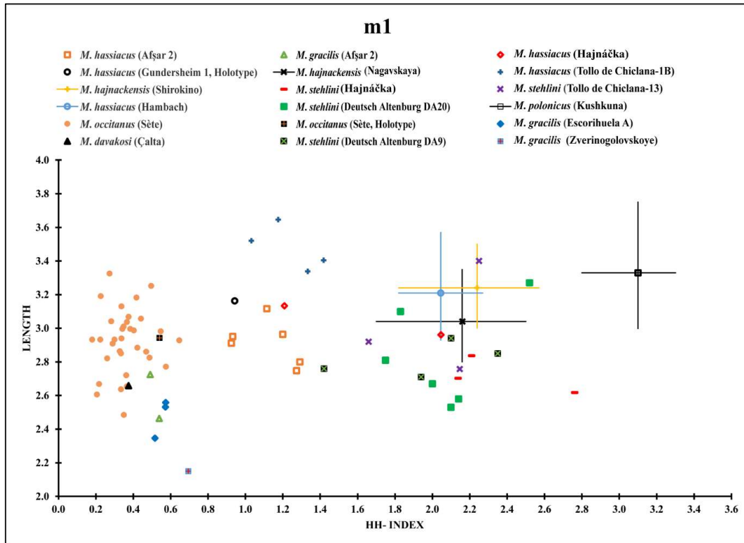
Figure 20. HH-index/L scatter plot of the m1 from M. hassiacus from Afsar 2, Gundersheim 1 (MN 16) (Heller, 1936), Hambach (Early Villanyian) (Mörs et al., 1998: figure 19, table 1), Hajnáčka (MN 16) (Fejfar, 1961, original assignment – M. hajnackensis ) and Tollo de Chiclana-1B (MN 15) (taken from illustration, Minwer-Barakat et al., 2008: figure 2); M. hajnackensis from Shirokino (MN 16) and Nagavskaya (MN 16) (Tesakov, 2004: tables 4.2, 4.3, assignment of the present authors – M. stehlini ); M. stehlini from Hajnáčka (Fejfar, 1961), Tollo de Chiclana-13 (MN 16) (taken from illustration, Minwer-Barakat et al., 2008: figure 3), Deutsch Altenburg DA20 (MN 16) and Deutsch Altenburg DA9 (Pliocene) (Rabeder, 1981, original assignment – M. kretzoi ); M. occitanus from Sète (MN 15) (Thaler, 1955; Holotype) and M. occitanus from Sète (additional material); M. gracilis from Afsar 2, Escorihuela A (MN 15) and Zverinogolovskoye (MN 15/16) (Mein et al., 1990; Pogodina and Strukova, 2016); M. davakosi from Çalta (MN 15) (Şen, 1977); M. polonicus from Kushkuna (MN 16) (Tesakov, 2004). Measurements were made in millimetres.
