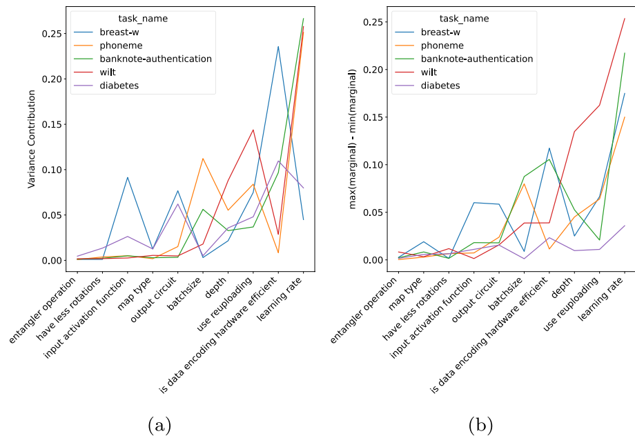
Fig. 5 The marginal contributions per dataset are presented as a the variance contribution and b the difference between the minimal and maximal value of the marginal of each hyperparameter. The hyperparameters are sorted from the least to the most important using the median. We distinguish from the plot 3 primary levels of importance
