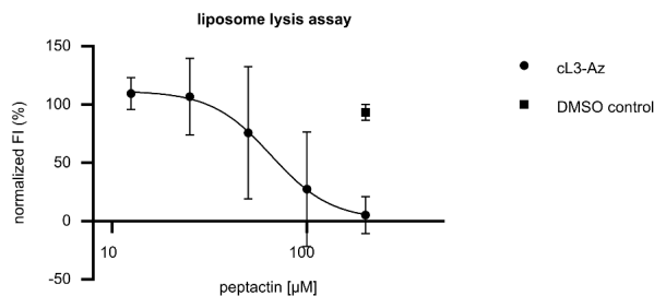
Figure S14. Normalized FI data of the inhibition experiment displayed in fig 5b. Datapoints are normalized to the average values of the conditions where no Ab was present ( min ) and only Ab was present ( max ). Data was normalized using (FI - min) / (max - min) * 100\% . The DMSO control is to check for activity in the absense of cL3-Az. Datapoints are displayed and the fitted model is the black line. Graphpad Prism version 9.3.1 was used for model fitting using a non-linear dose vs response curve with four parameters least squares fit. IC50: 65 , CI confidence interval (%) IC50: ND, R^2 : 0.62.
