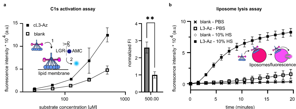
Figure 4. Activation of complement on lipid bilayer surfaces. a) DBCO Liposomes conjugated to cL3-Az can activate the C1s proteases. Activation of C1s (1) results in cleavage of LGR-AMC and an increase in fluorescence (2). Raw fluorescence data is shown in the left. On the right, the fluorescence data with baseline activity of C1s in the presence of blank liposomes is set to 1, and displays a significant difference to the upregulated activity by cL3 modified liposomes (**, p < 0.01 , unpaired t-test, Graphpad Prism version 9.3.1.) (One batch of conjugated liposomes, samples measured in triplicate). b) DBCO liposomes conjugated to cL3-Az can be lysed via complement activation, resulting in an increase in fluorescence (conjugation was performed twice, on separate days and samples were measured in triplicate each time). Liposomes were exposed to 10% human serum (HS) in PBS and fluorescence was measured immediately after. Blank controls in a,b are liposomes that present 1% DBCO, but are not conjugated to cL3-Az.
