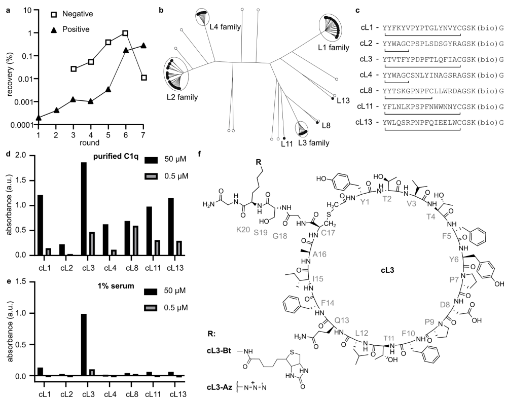
Figure 2. RaPID selection, sequence analysis and peptide screening. a) qPCR quantifying DNA recovery after each selection round. cDNA conjugated peptides were either incubated with SCgC1q-presenting beads (positive) or beads without protein (negative). b) Phylogenetic tree representation of the top 100 sequences. c) Representative sequences obtained from each cluster in b . Lines connecting N-terminal tyrosine and cysteine denote the position of cyclization, and (bio) denotes the C-terminal lysine analogue that was modified with biotin. d,e) ELISAs where peptides were incubated with either purified C1q or human serum (1% in RPMI medium). Single datapoints are shown. Peptides were incubated at two concentrations 50 \mu M and 500 nM, either with purified C1q or 1% human serum. f) Structure of cL3, which was modified with either a biotin (cL3-Bt) or azide (cL3-Az) moiety.
