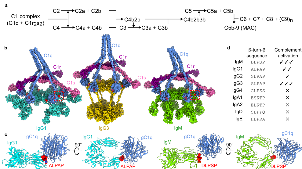
Figure 1. The classical complement pathway is initiated by defined structural motifs. a) Overview of the classical complement pathway. b) CryoEM-derived structures of antibody-C1 complexes. The interfaces between the gC1q domains and antibodies are highlighted in red. Structures were built into maps with accession codes EMD-4232, EMD-16241, and EMD-4878 (IgG1, IgG3 and IgM, respectively). c) Structures of the interfaces (dashed boxes in b ) between gC1q and ALPAP (IgG1 and IgG3; left) and DLPSP (IgM; right). d) Sequence comparison of the \beta -turn- \beta motif of human antibody (sub)classes, and their ability to activate complement (24).
