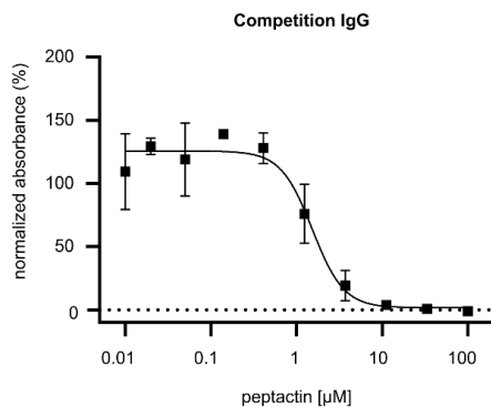
Figure S18. Normalized absorbance data as described in fig 6b. Datapoints are shown and was fitted (black line) using Prism version 9.3.1 for model fitting using a non-linear dose vs response curve with four parameters least squares fit. Competition with IgG: IC50: 1.5, CI confidence interval (%) IC50: 1.01-2.13 , R^2 : 0.94.
