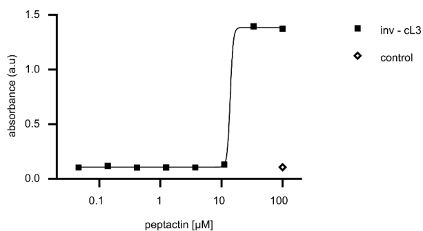
Figure S17. Absorbance data as described in fig 6a. Datapoints are shown and was fitted (black line) using Graphpad Prism version 9.3.1 for model fitting using a non-linear dose vs response curve with four parameters least squares fit. EC_{50} : 13.9, CI confidence interval (%) EC_{50} : ND, R^2 : 0.99.
