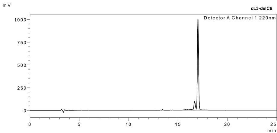
Figure S8. Analytical HPLC trace.
