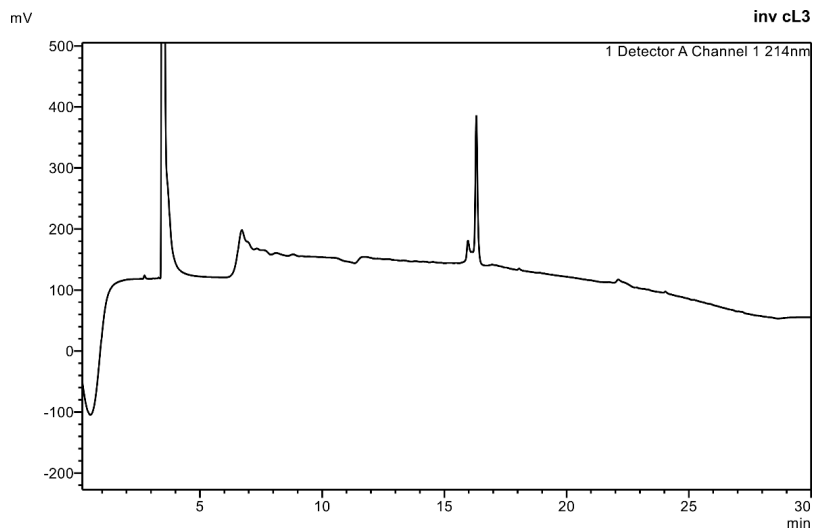
Figure S16. Analytical HPLC trace.
