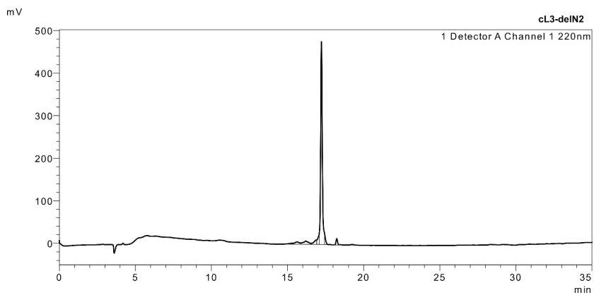
Figure S10. Analytical HPLC trace.
