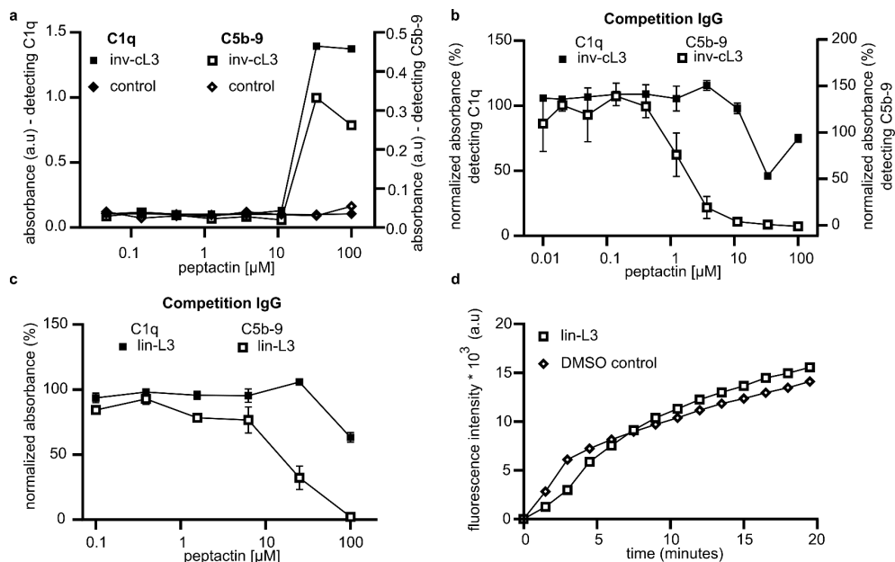
Figure 6. cL3 variants effect on complement modulation. a) ELISA determining the activation of complement in 1% human serum by azide modified inv-cL3 detecting C1q and C5b-9 (technical singlet). b) Competition ELISA showing inv-cL3 inhibiting C1q and C5b-9 deposition by blocking binding to pooled IgG (two technical replicates). c) Competition ELISA showing lin-L3 inhibiting C1q and C5b-9 deposition by blocking binding to pooled IgG (two technical replicates). d) The ability of lin-L3 to inhibit complement activation by IgG was assessed in liposome lysis assays (single experiment shown, experiment was repeated twice, once at 10 min pre-incubation, once at 1 hour).
