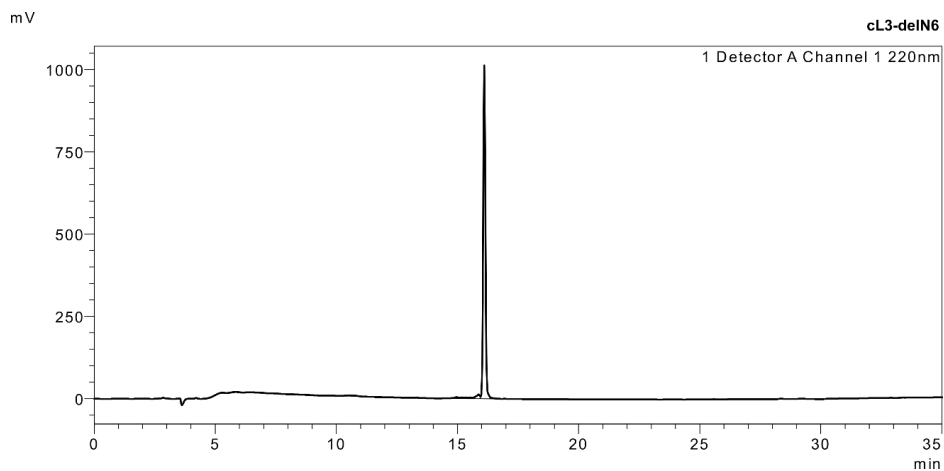
Figure S12. Analytical HPLC trace.
