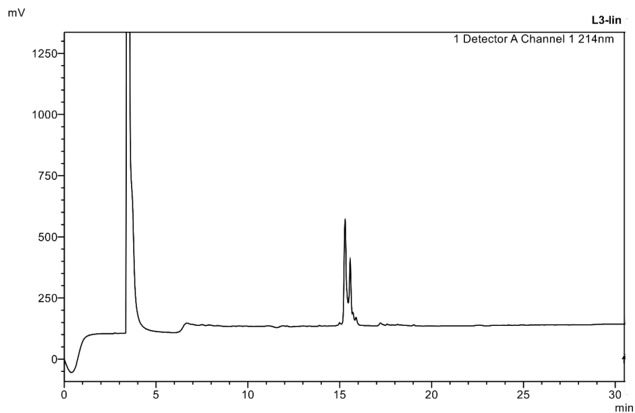
Figure S19. Analytical HPLC trace.
