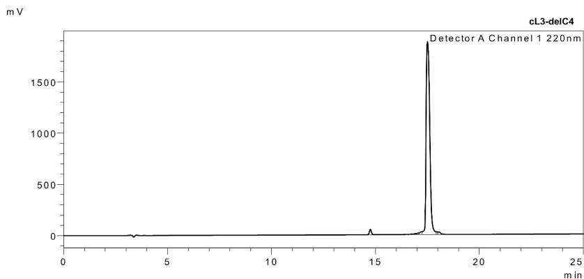
Figure S7. Analytical HPLC trace.
