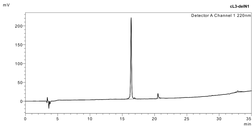
Figure S9. Analytical HPLC trace.
