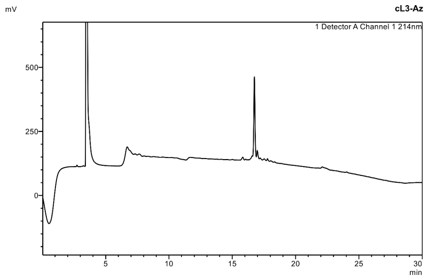
Figure S3. Analytical HPLC trace.
