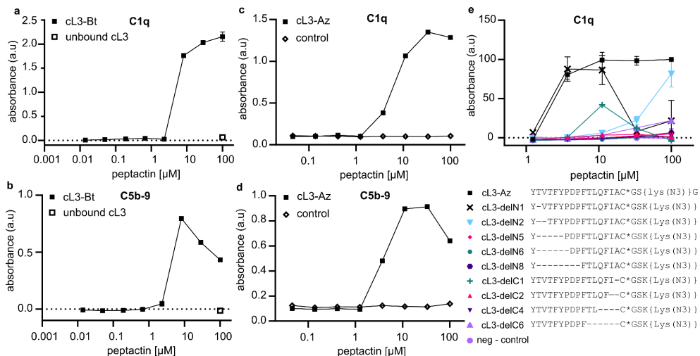
Figure 3. Activation of complement via C1q binding to cL3. a) representative ELISA detecting C1q was performed to evaluate the ability of cL3-Bt to bind C1 from 1% human serum in RPMI medium (two technical replicates). See Fig. S2 for fitted models of the data and additional technical replicates collected on different days. The control consists of unbound cL3, but no streptavidin, indicating the necessity of the streptavidin monolayer to recruit C1q. b) ELISA detecting C5b-9 deposition to evaluate complement activation by cL3-Bt (two technical replicates). In both a and b , streptavidin-coated plates are used and cL3-Bt is bound directly the biotin moiety. c) As in a , but this time the cL3-Az variant was immobilized on the plate using a DBCO-biotin linker that was co-incubated with the cL3-Az peptide on the plate for 1 hour at 37 °C. Thereafter, excess peptide was washed away and peptides were incubated with 1% human serum in RPMI medium before C1q was detected. Control is the condition with only biotin-DBCO linker present. See Fig. S4 for fitted model of the data. d) As in c , but this time with detection of C5b-9. e) Deletion mutants of cL3 as in c : binding was assessed to determine recruitment of C1q from 1% human serum in PRMI. Lys(N3) denotes the lysine residue with the sidechain amine replaced by an azide, and * denotes that the cysteine has been cyclized via the N-terminal chloroacetyl modification. c, d display the data of one titration of cL3-Az. Further replicates of cL3-Az are contained in e , which displays technical duplicates.
