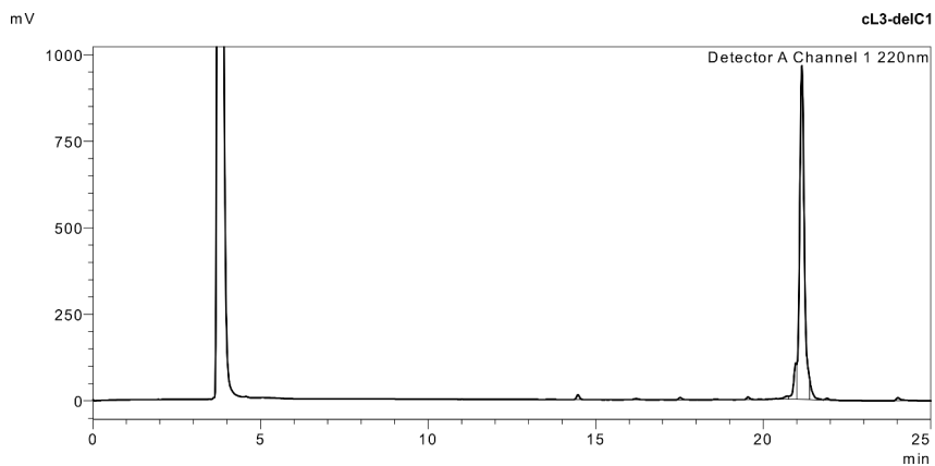
Figure S5. Analytical HPLC trace.
