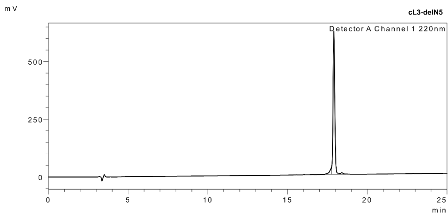
Figure S11. Analytical HPLC trace.
