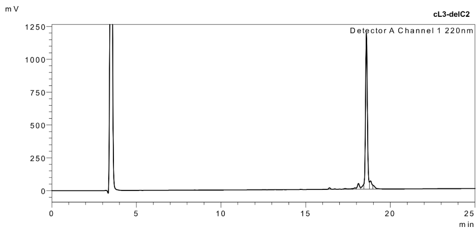
Figure S6. Analytical HPLC trace.
