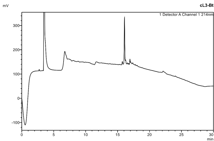
Figure S1. Analytical HPLC trace.
