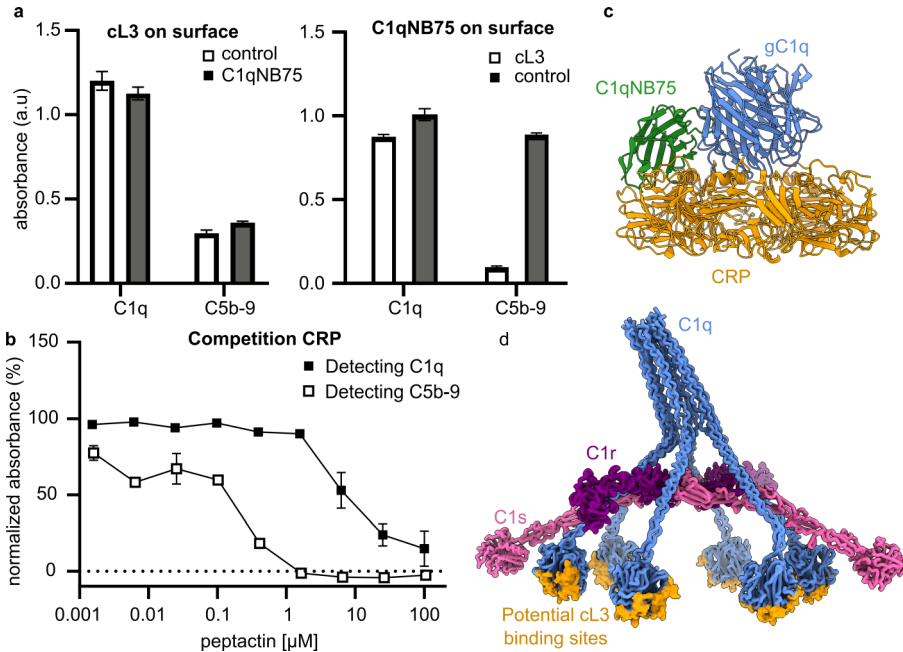
Figure 7. Competition assays between cL3 and C1q binders. a) Competition ELISAs where either cL3-Bt (left) or C1qNB75 (right) are immobilised and competed against solution phase C1qNB75 (100 nM) or cL3 (20 \mu M), respectively, in the presence of 1% human serum. Binding of complement component C1q and deposition of C5b-9 was measured. (three technical replicates) b) ELISAs determining cL3-mediated inhibition of C1q binding and C5b-9 deposition by CRP. 1% human serum was incubated with cL3-Az before adding to the wells containing CRP. Samples are normalized to the DMSO control (maximal signal, 100%) and no serum samples (minimal signal, 0%). (two technical replicates) c) Binding locations of CRP (orange) and C1qNB75 (green) on gC1q (blue). d) C1 complex showing potential cL3 binding locations (orange).
