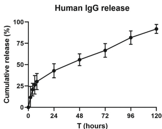
Figure 3. In vitro human IgG release from 25% P407 hydrogel. Hydrogels loaded with 100 \mu g IgG were loaded in 15 mL Falcon tubes and 37 °C PBS pH 7.4 was layered on top to serve as release medium. At the indicated time-points, release medium was collected and IgG levels were quantified with ELISA. Results are shown as mean \pm SD for two independent experiments, with N = 6 in total.
