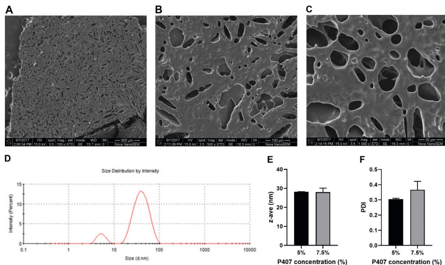
Figure 2. SEM images reveal the porous structure of 25% P407 hydrogel at 100× (A), 500× (B) and 1000× (C) magnification. A representative histogram for the micelle size is depicted in (D; left peak at 5 nm) and the average size (z-ave) and PDI are depicted in (E) and (F), respectively. Results are shown as mean \pm SD for a triplicate measurement.
