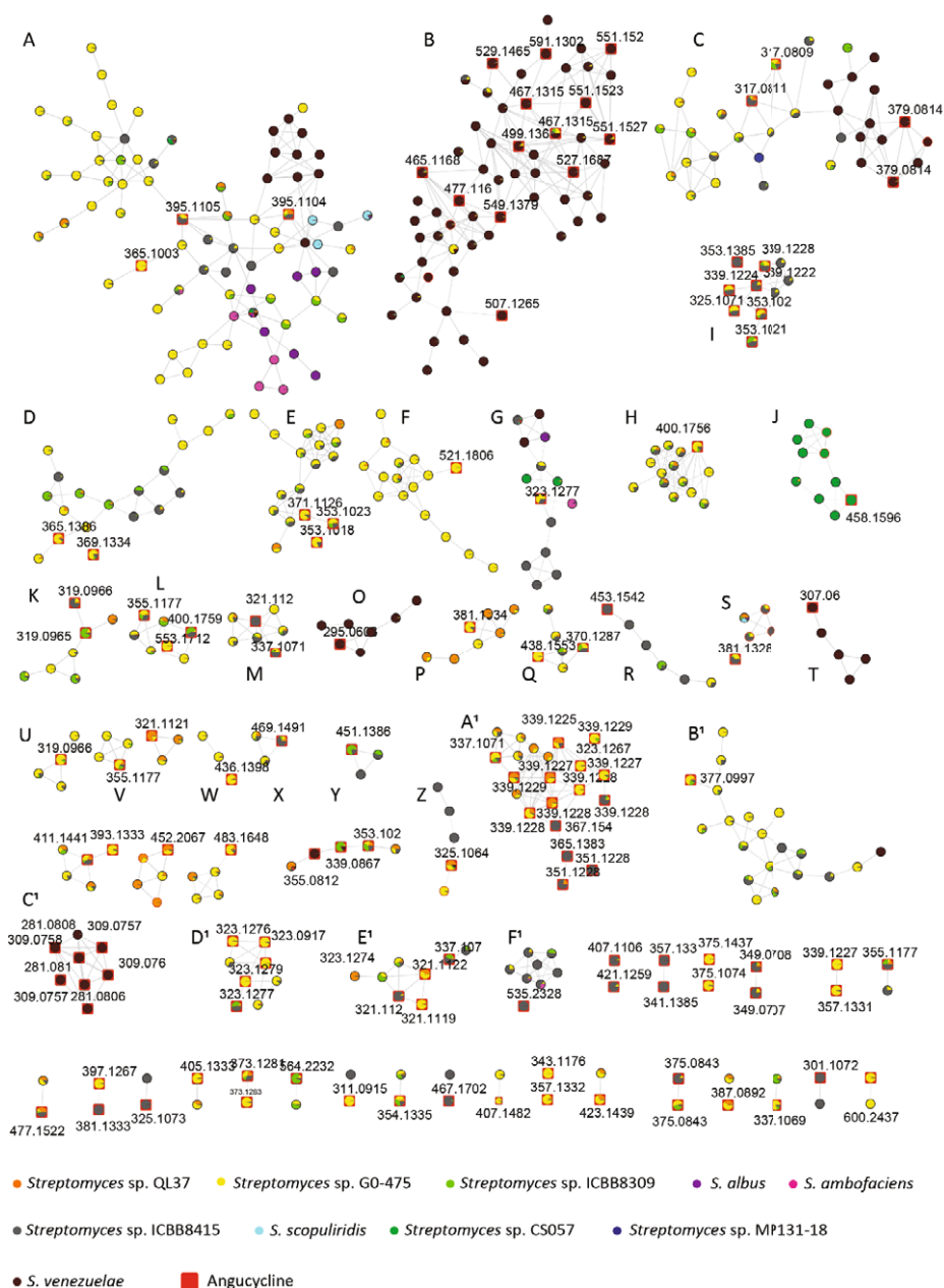
Figure 2. Molecular network representing the molecules identified in the crude extracts of the angucycline-producer strains by GNPS-molecular networking and SIRIUS in the extracts. Colors of the pie charts correspond to the relative abundance of the chromatographic peaks in each strain. Red square represents features identified as angucyclines by CANOPUS. The edge connects two nodes when the cosine similarity score is above 0.6.
