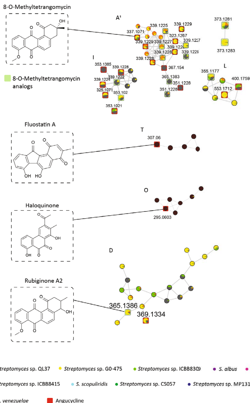
Figure 3. Spectral families containing the dereplicated angucyclines and analogues identified by GNPS-molecular networking of culture extracts. Colours of the pie charts within the nodes correspond to the relative abundance of the ions in the different strains. Red square represents features identified as angucyclines by CANOPUS. Green squares represent features identified as analogues.
