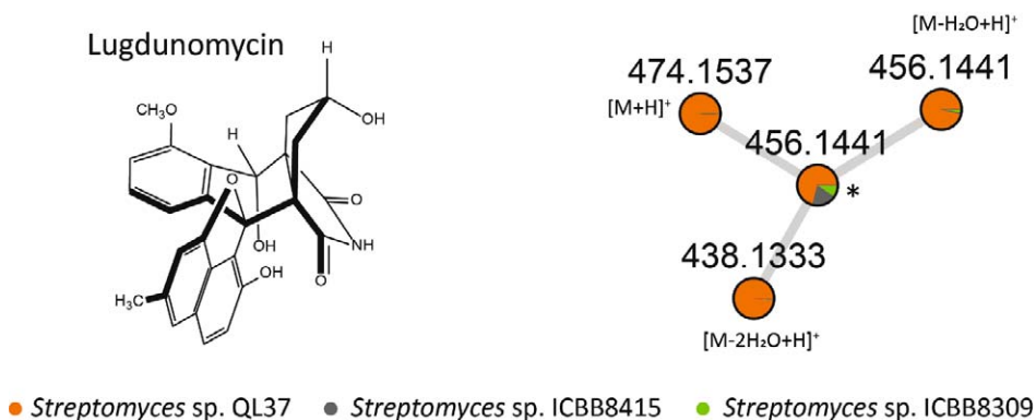
Figure S3. Identification of lugdunomycin-like molecules using molecular networking. The structure of lugdunomycin is depicted on the left. On the right, the lugdunomycin network is shown, consisting of four nodes. The three nodes with the 7.1-min retention time are exclusively present in the Streptomyces sp. QL37 extract (orange). The fourth node ( m/z 456.1441, retention time 6.8 min, highlighted with a star) is predominantly found in Streptomyces sp. QL37 and corresponds to a lugdunomycin isomer.
