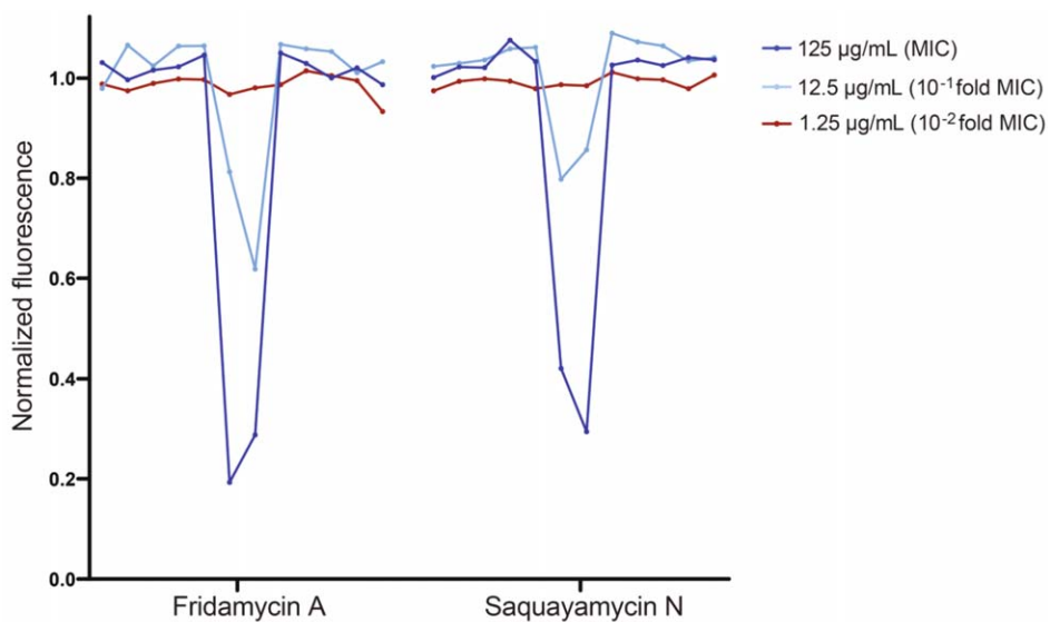
Figure S23. Results of the resazurin reduction assay for the purified saquayamycin N ( 1 ) and fridamycin A ( 2 ) against B. subtilis 168. Compounds were tested in 125 µg/ml, 12.5 µg/ml and 1.25 µg/ml concentration. Note, that the MIC and sub-MIC concentration (12.5 µg/ml) resulted in the drop of fluorescence.
