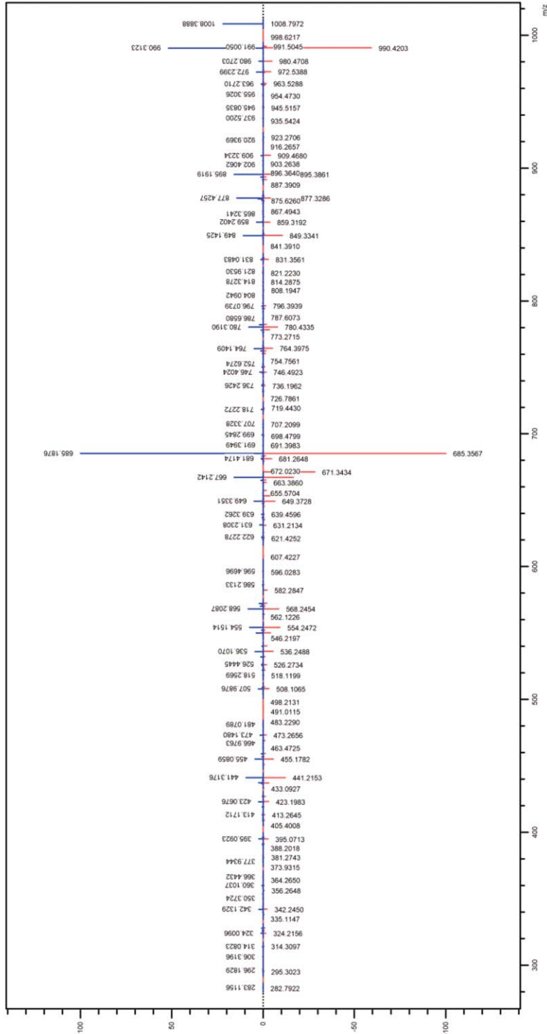
Figure S6. Direct MS/MS comparison of surfactin Leu/Ile 7 C13 from the extract of Bacillus sp. 90A-23 with surfactin Leu/Ile 7 C13 spectral from GNPS spectral library (CCMSLIB00000006885).
