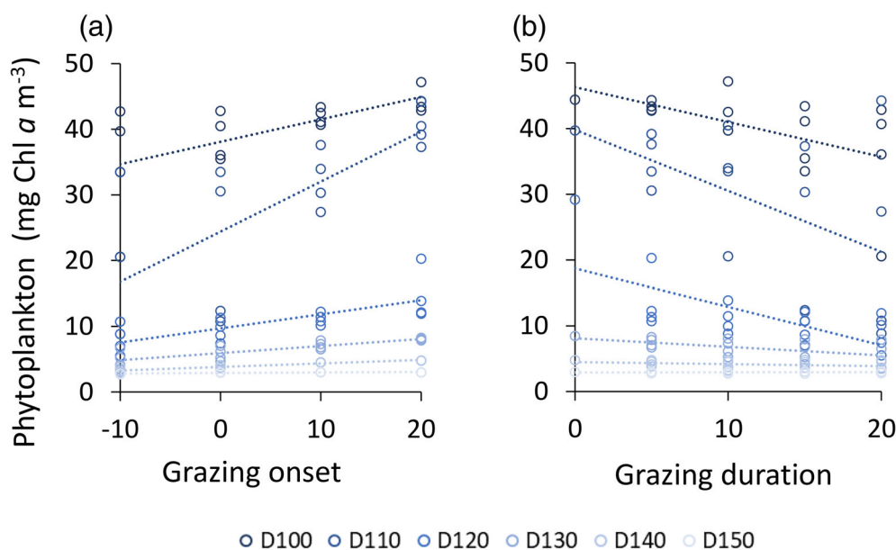
Fig. 5. The 25-yr average summer pelagic phytoplankton biomass (mg chlorophyll a [Chl a ] \text{m}^{-3} ) along a gradient of epiphyton shading curve midpoints (day [D] 100–150; blue shades) in presence of a grazing event and under the control temperature scenario relative to the (a) onset of the grazing period and (b) duration of the grazing event.
