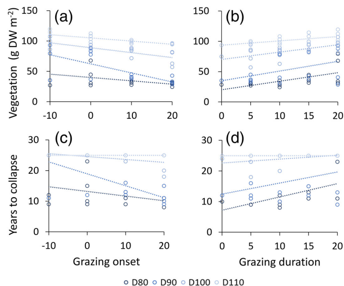
Fig. 4. Response of submerged macrophyte biomass and resilience in the warmer winter temperature scenario. The 25-yr average summer biomass of macrophytes (g dry weight [DW] \text{m}^{-2} ) relative to (a) timing of the grazing period, and (b) duration of the grazing event. Years until macrophytes disappear during the growth period from the model lake along a gradient of epiphyton shading curve midpoints (day [D] 80–110; blue shades) in response to (c) the relative onset of the grazing period and (d) the duration of the grazing period.
