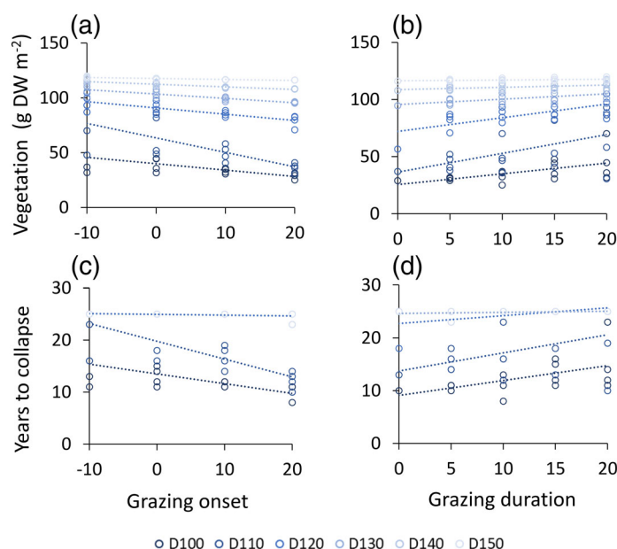
Fig. 3. Scatter plots along a gradient of epiphyton shading curve midpoints (day [D] 100–150; blue shades) in presence of a grazing event in the control temperature scenario. (a) The 25-yr average summer biomass of macrophytes ( \text{g dry weight [DW] m}^{-2} ) against onset of the grazing period relative to the midpoint of the shading curve. The spread of points along the y-axis for each shading curve set reflects the influence of the duration of the grazing period (5, 10, 15, and 20 d). (b) The same 25-yr average summer biomass of macrophyte data against the duration of the grazing event. The spread of points along the y-axis for each shading curve set reflects the relative onset of the grazing period (–10, 0, 10, and 20 d). (c) Years until macrophytes disappear during the growth period from the model lake in response to the relative onset of the grazing period. (d) Years until macrophytes disappear during the growth period from the model lake in response to the duration of the grazing period.
