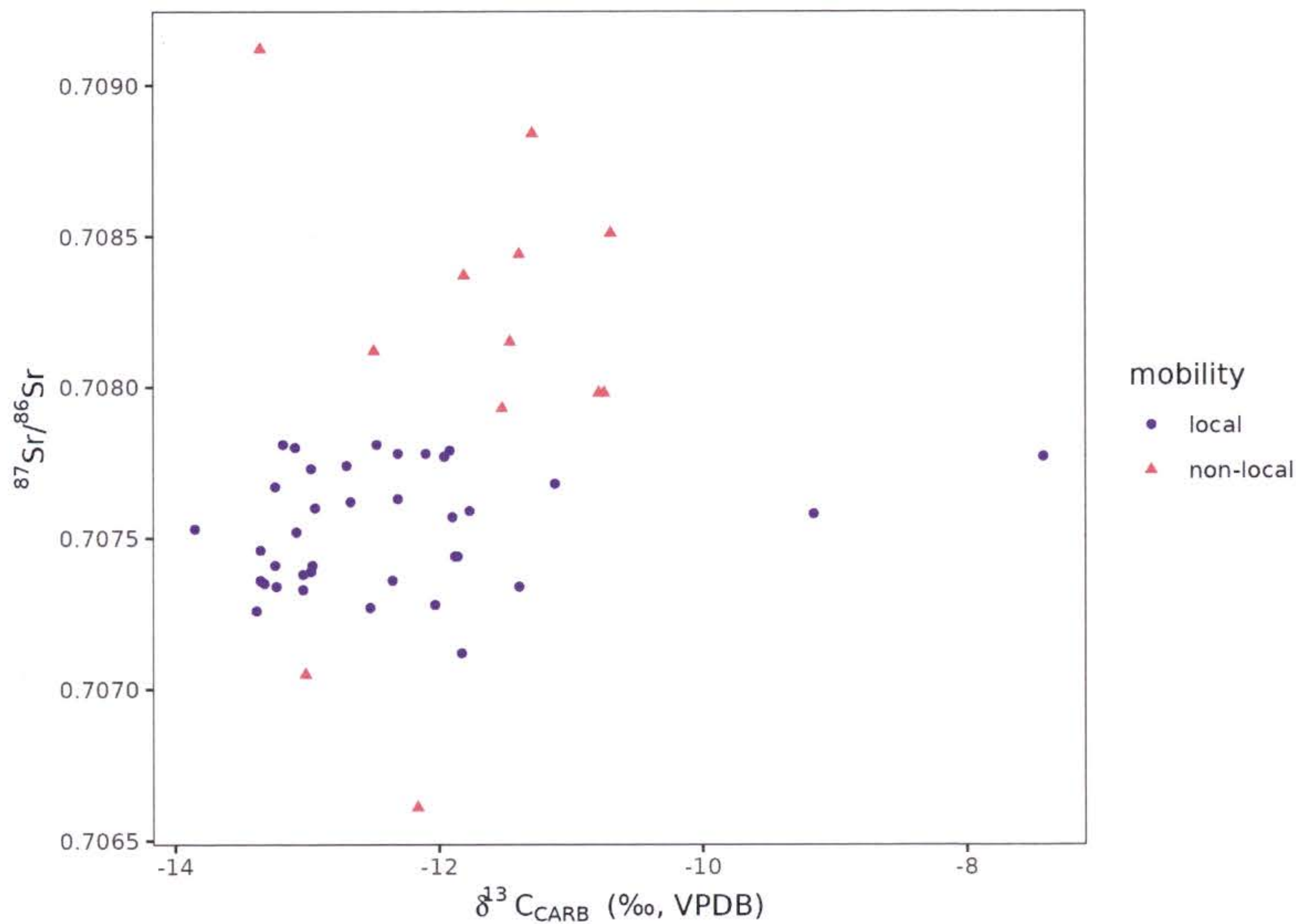
Fig. 3 Tombos locals versus non-locals carbon values compared.
