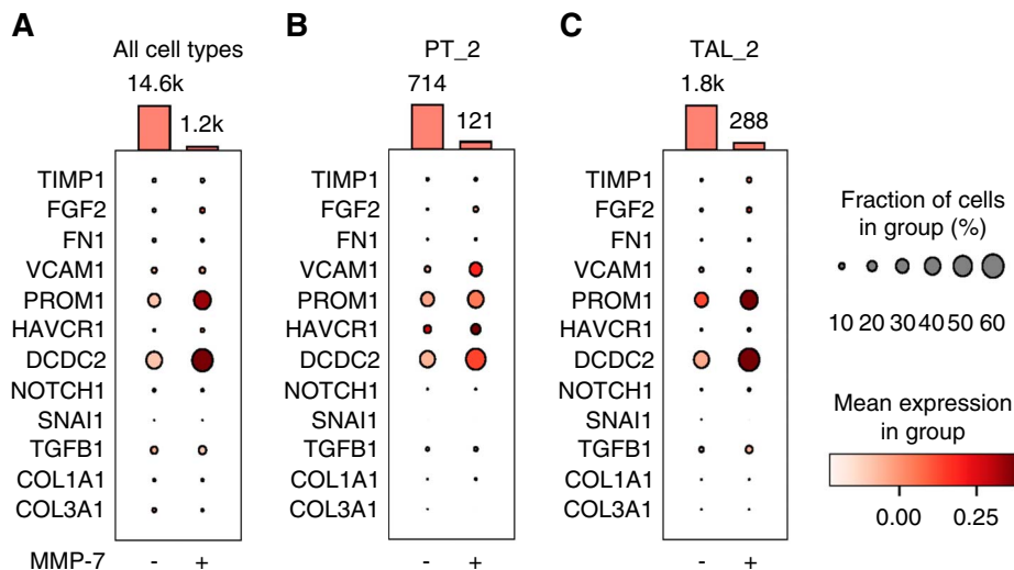
Figure 8. Profibrotic profile of MMP-7 expressing cells. Single-nucleus RNA sequencing of human kidneys recognizes a significantly increased profibrotic expression profile in (A) MMP-7-positive cells for all cell types and those cell types with an increased MMP-7 expression, including (B) PT epithelial cells and (C) TAL cells. COL1A1, collagen type I alpha 1 chain; COL3A1, collagen type III alpha 1 chain; DCDC2, doublecortin domain containing 2; FGF2, fibroblast growth factor 2; FN1, fibronectin 1; HAVCR1, hepatitis A virus cellular receptor 1; NOTCH1, notch receptor 1; PROM1, prominin-1; SNAI1, snail family transcriptional repressor 1; TIMP1, tissue inhibitor of metalloproteinases 1; TGFB1, TGF beta 1; VCAM1, vascular cell adhesion molecule 1.
