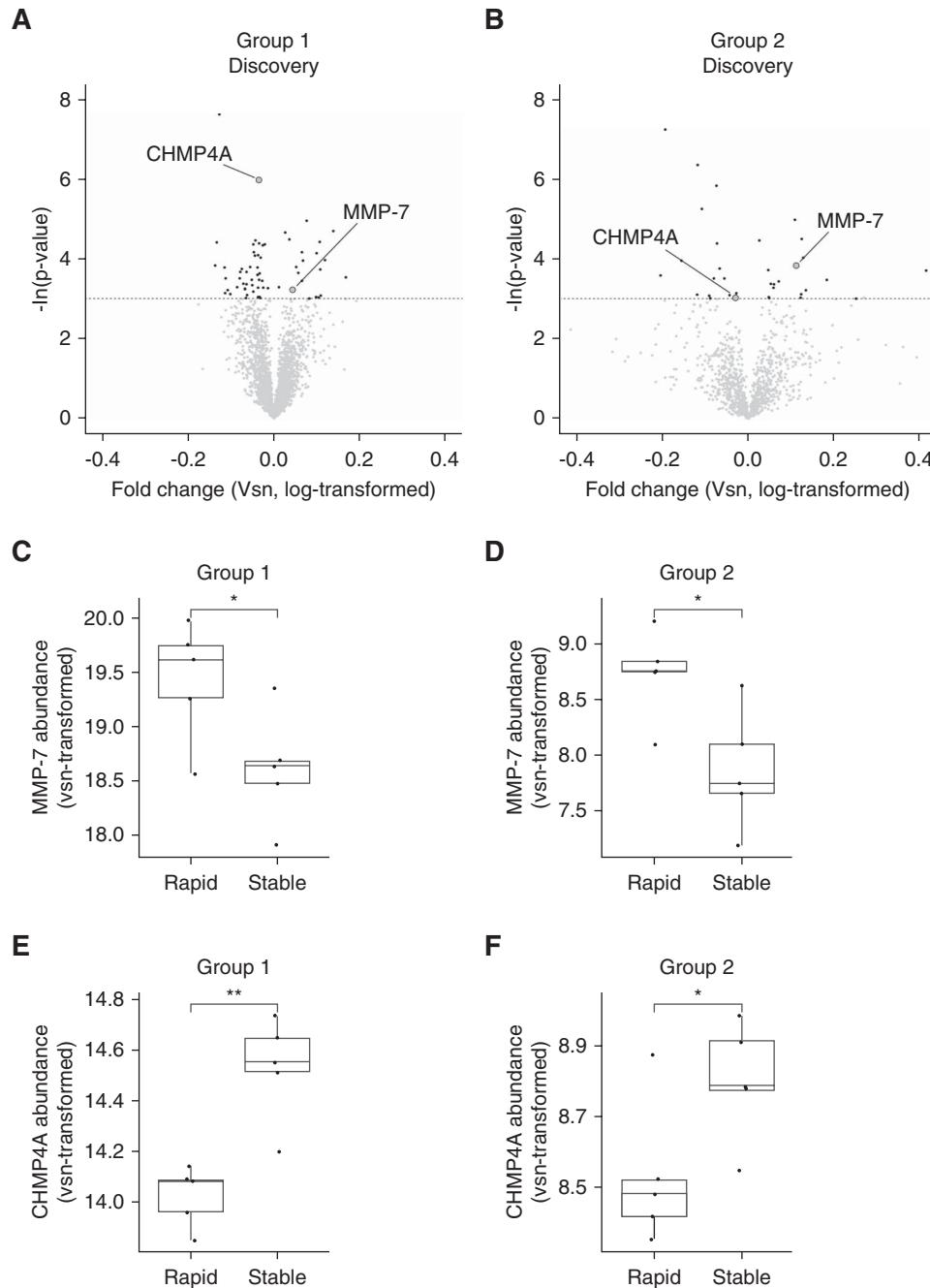
Figure 4. Identification of uEV-MMP-7. Volcano plots for the comparison of protein abundance in isolated uEVs of patients with rapid disease progression versus stable disease in (A) group 1 and (B) group 2. X-axis depicts vsn-normalized abundance ratio (rapidly progressive/stable), which includes a log transformation. Y-axis depicts naturally log-transformed P values of the Student t test, with cutoff at -\ln(0.05) . Significantly different proteins ( P < 0.05 ) are marked in darker gray. Abundance of biomarker candidates (C and D) MMP-7 and (E and F) CHMP4A in the MS/MS experiments of groups 1 and 2. Abundances were vsn-normalized, which includes log transformation. * P < 0.05 , ** P < 0.01 by the Student t test. CHMP4A, charged multivesicular body protein 4a; MMP-7, matrix metalloproteinase 7.
