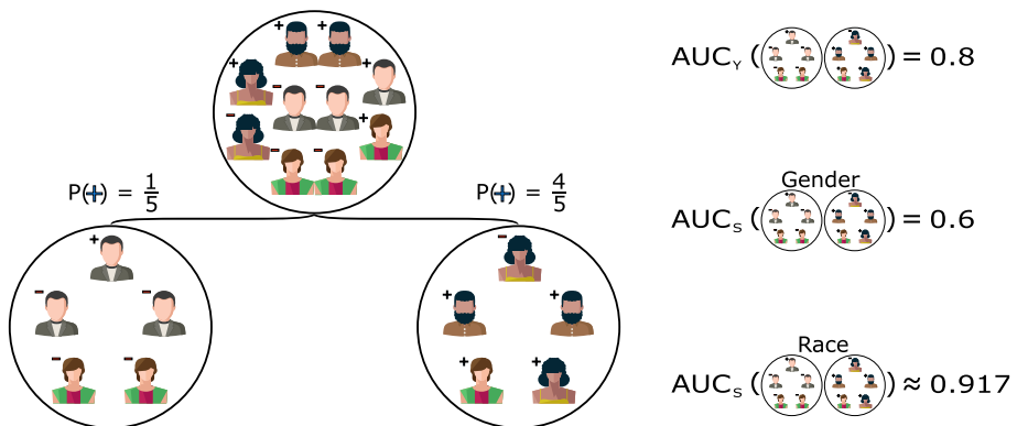
Fig. 1 Computing necessary AUC values for split evaluation, with 2 sensitive attributes ( race and gender ). Instances pertaining to a node are assigned its respective positive class probability as their Z scores, denoted above each child node
