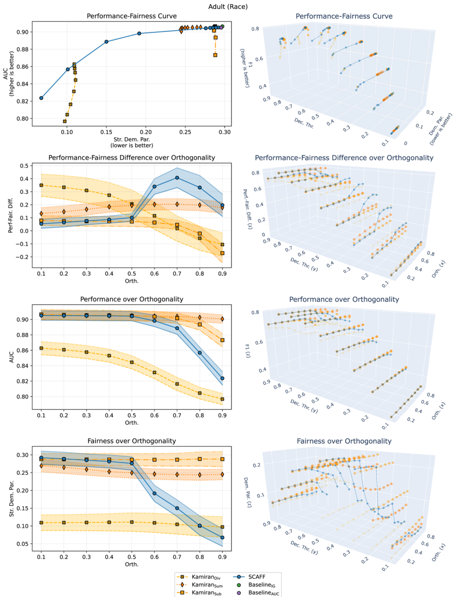
Fig. 2 Performance-fairness in the binary sensitive attribute setup Adult (Race)
