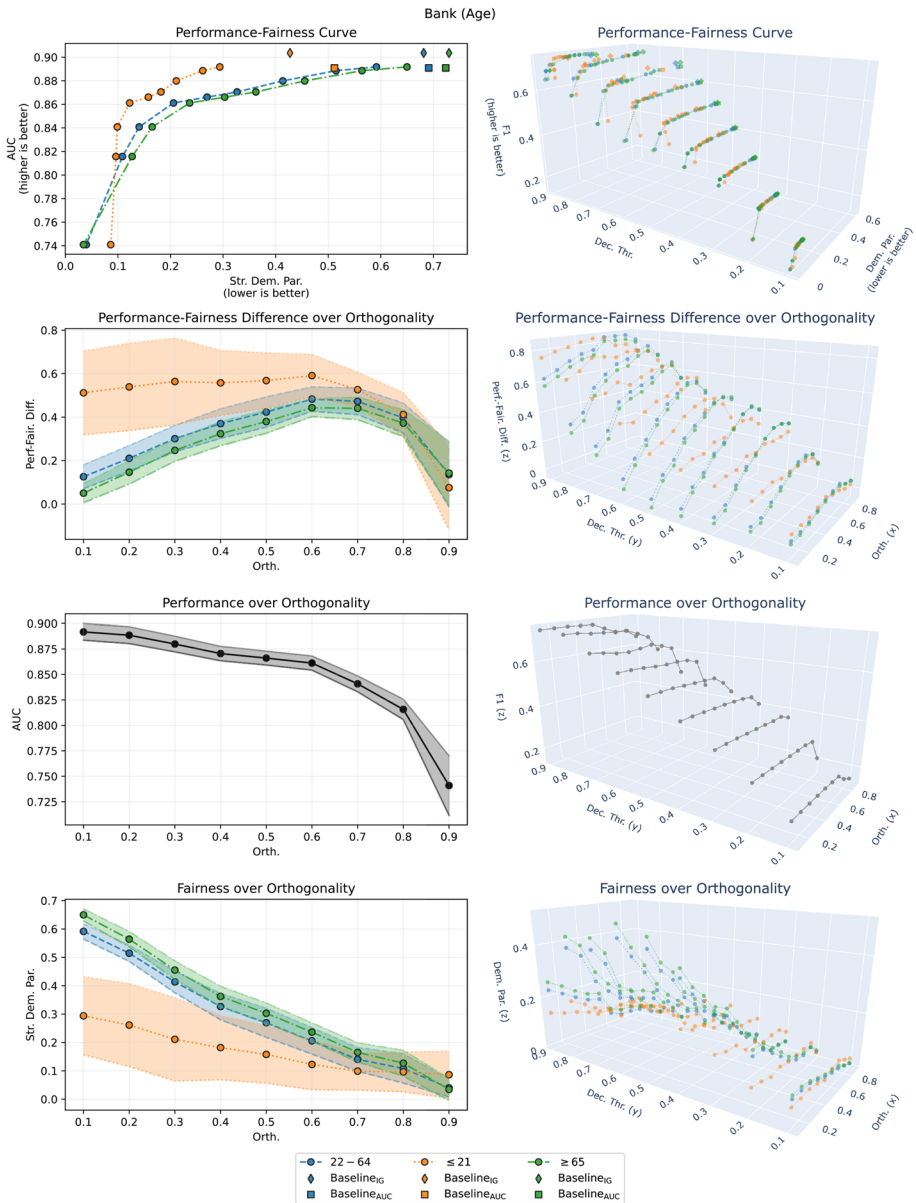
Fig. 5 Performance-fairness in the multicategorical sensitive attribute setup Bank (Age)
