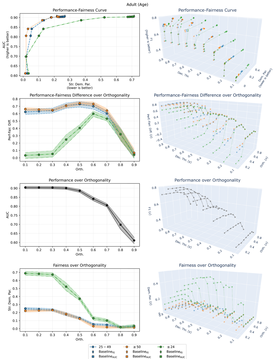
Fig. 4 Performance-fairness in the multicategorical sensitive attribute setup Adult (Age)
