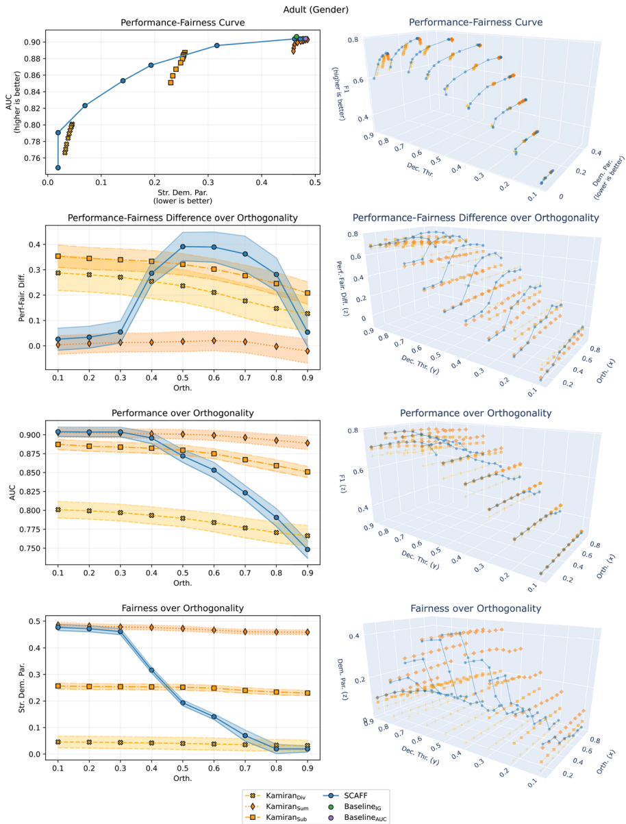
Fig. 3 Performance-fairness in the binary sensitive attribute setup Adult (Gender)
