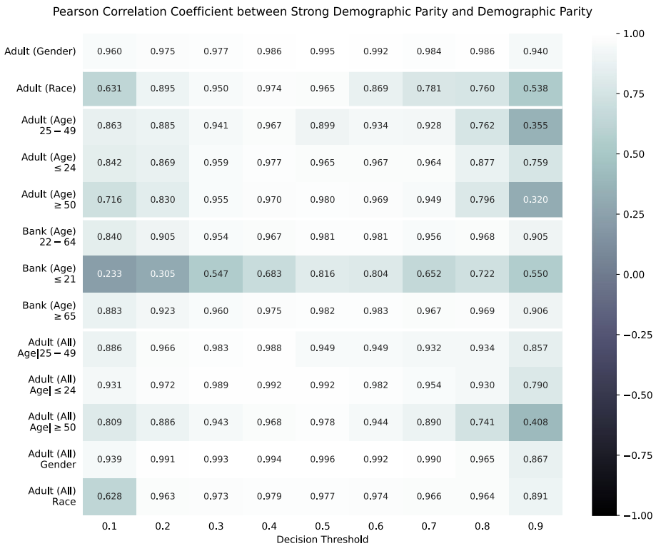
Fig. 7 Pearson correlation coefficient between strong demographic parity and demographic parity at different decision thresholds. Each cell corresponds to the correlation between the fairness measures over orthogonality \Theta across all folds
