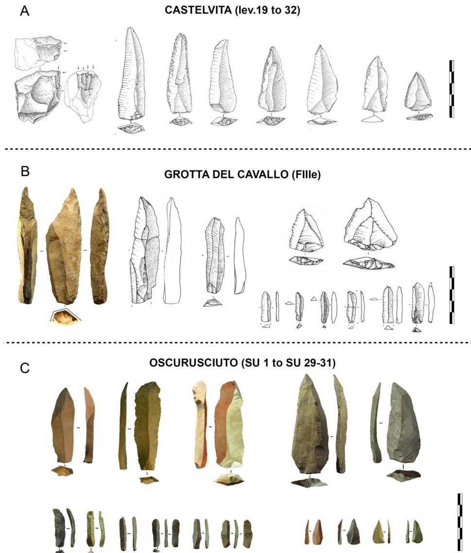
Fig. 21 Visual comparison of a selection of end-products from Oscurusiuto and two Late Middle Paleolithic sites attributed to the “Evolved Mousterian.” A Grotta di Castelcivita (Drawings by G. Fabbri, University of Siena.) B Grotta del Cavallo after modified after Carmignani & Sarti 2018. C Oscurusiuto
