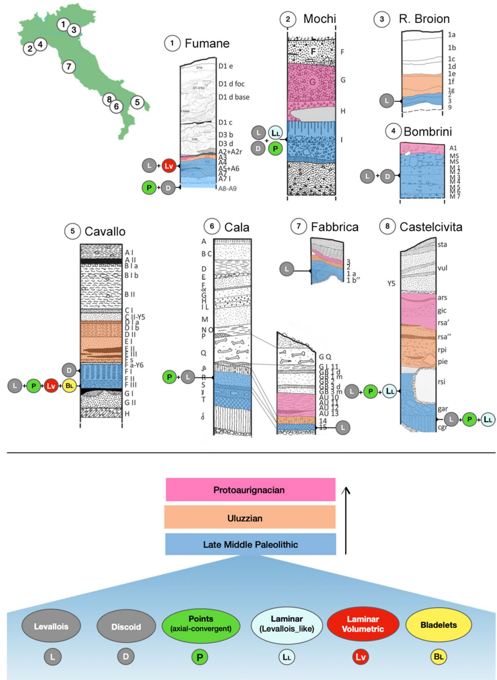
Fig. 1 Stratigraphic sequences with Mousterian, Uluzzian, and Protoaurignacian. 1 Fumane modified from Tagliacozzo et al., 2013. 2 Mochi modified from De Lumley, 1969. 3 R. Broion modified from Peresani et al., 2019. 4 Bombrini modified from Riel-Salvatore and Negrino, 2018. 5 Cavallo modified from Palma di Cesnola, 1964. 6 and 8 La Cala and Castelvita modified from Gambassini, 1982. 7 La Fabbrica modified from Villa et al., 2018
