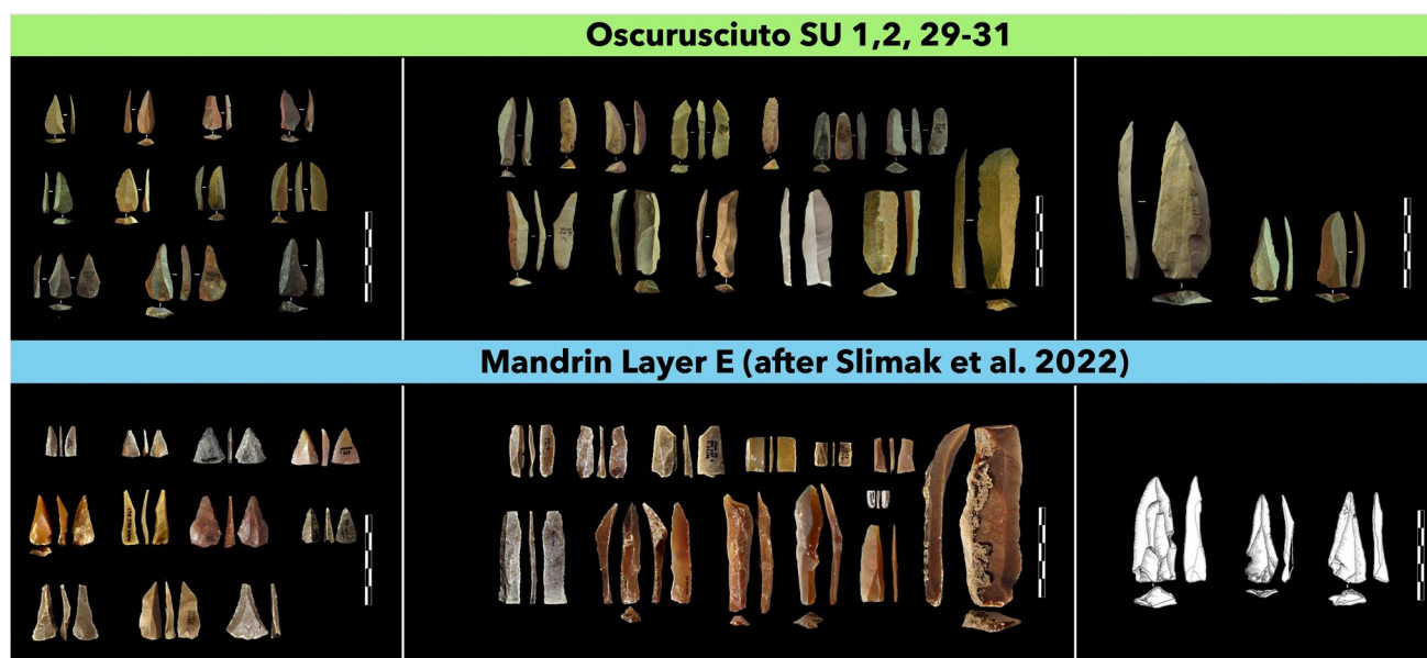
Fig. 24 Comparison between Oscursciuto (SU1 to SU29–31) and Mandrin. Adapted from Slimak et al., 2022
