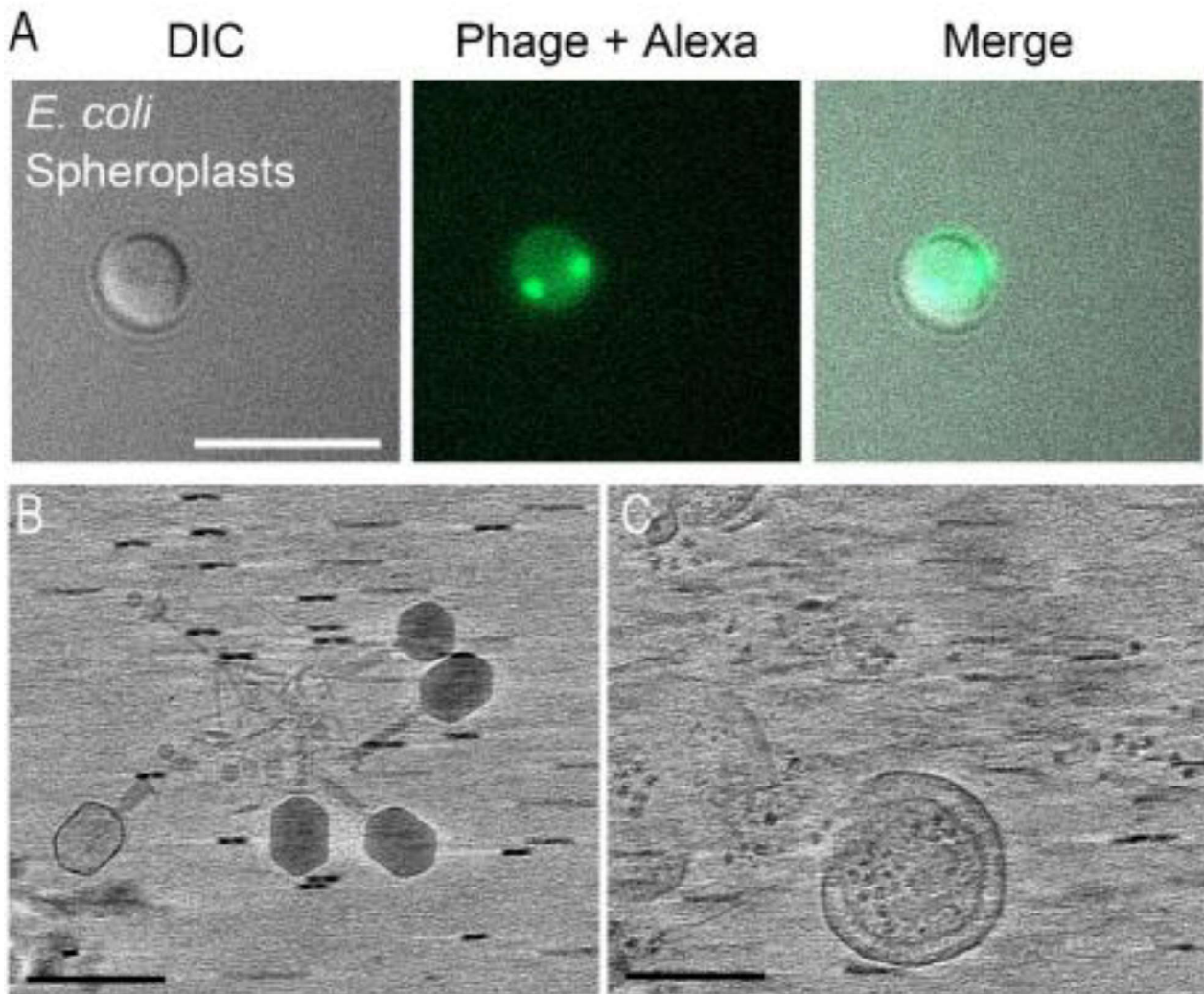
Figure S3. Heterogeneous appearance of E. coli spheroplasts with phage T4. (A) E. coli strain ET8 spheroplasts were imaged 24 hours after inoculation with phage T4 that were previously dyed with Alexa Fluor™ 488 NHS-Ester. The CWD cells did not lyse and phages surrounded the cells as indicated by fluorescent green dots. Scale bars represent 10 \mu m. (B) Four unattached phages with a full capsid head and one with an empty capsid head. (C) Image of spheroplast fragments taken from the same tomogram as panel B. Phages were in close proximity to these fragments but not attached. Scalebars represent 200 nm.
