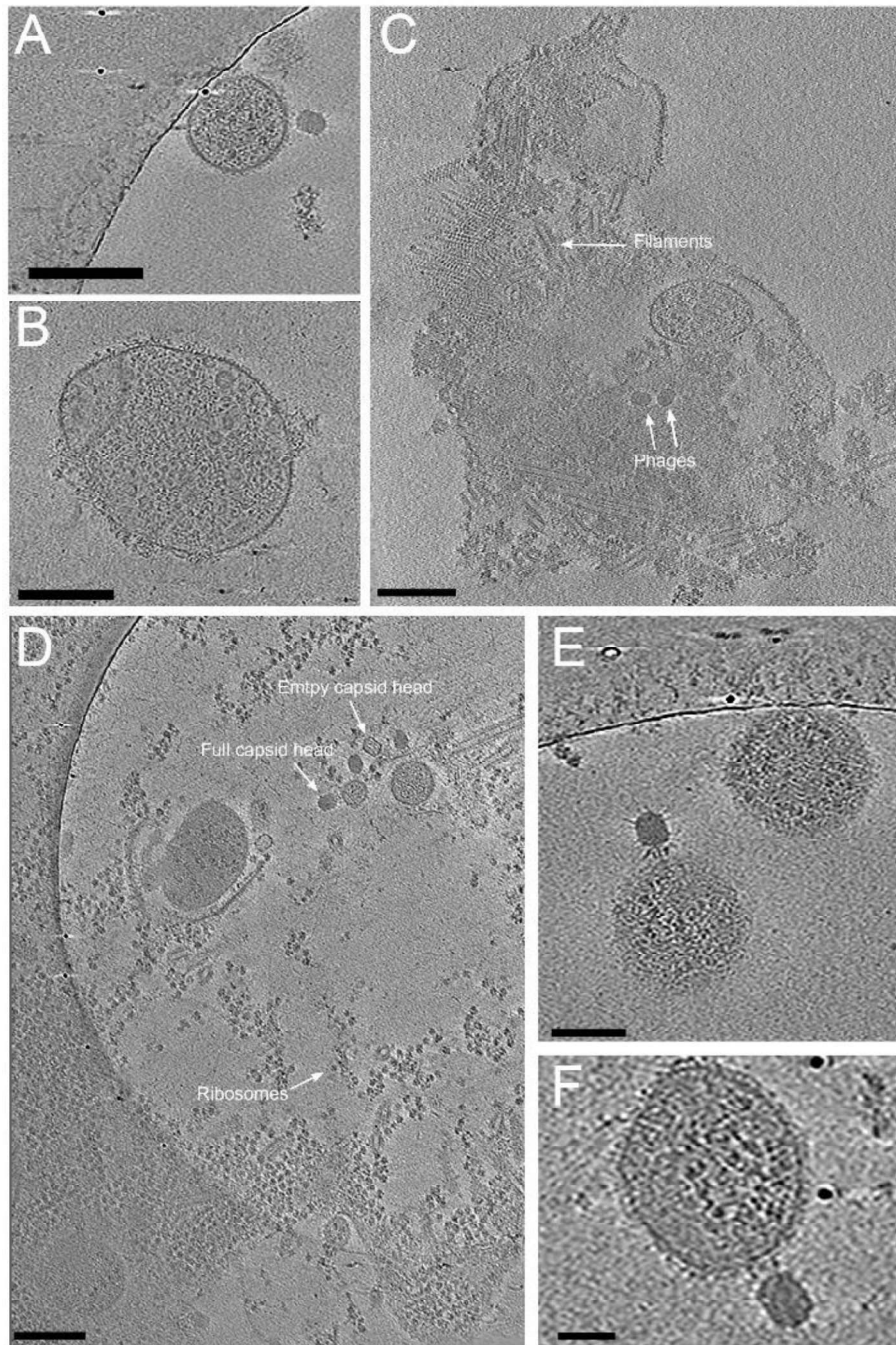
Figure S4. Phage \Phi 29 can attach to B. subtilis protoplasts and produce progeny. (A) One \phi 29 phage attaching to a B. subtilis protoplasts. (B) A protoplast with ribosomes and filaments inside. (C) An exploding protoplast extruding phages, filaments and cell debris in the environment. (D) A protoplast exploding at the bottom and phages with full and empty capsid heads attaching to CWD cells at the top. (E) Phage \phi 29 with a retracted sheet in the process of ejecting DNA inside a protoplast. (F) Phage \phi 29 attaching to a protoplast. Scale bars represent 70 nm (panel A), 50 nm (panel E and F) and 200 nm (panel B, C and D).
