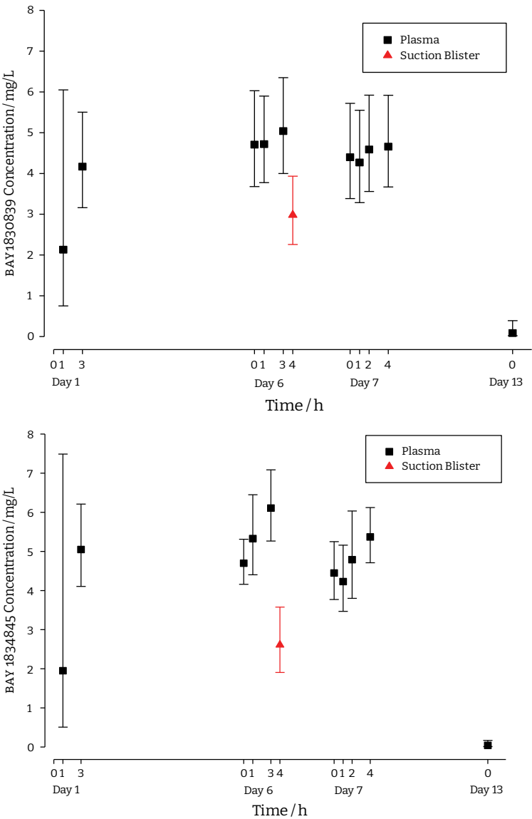
Supplementary Figure 4 Concentrations of BAY1830839 and BAY1834845 in plasma and suction blister fluid.
