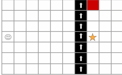
Figure 5.4: An illustration of the WindyGrid environment. The agent (smiley face) needs to navigate from the starting point to the given goal (star). There is the stochastic wind that will (black column with up arrows) blow the agent up and the agent gets a penalty when it reaches the trap (red cell).
