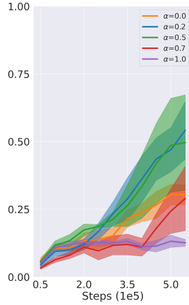
Figure 3.8: Performance of MoReFree with different values of \alpha in Push (hard).
