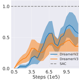
Figure 3.16: Performance of DreamerV2 and V3 on episodic Sawyer Door task. SAC can solve the task in 200k steps, while after 1 million steps MBRL is still not able to steadily solve the task.
