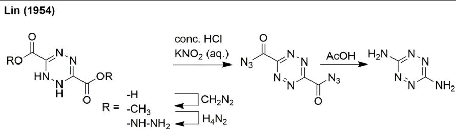
Scheme 5: An example of developments into symmetrical tetrazines by modification of existing tetrazines.
