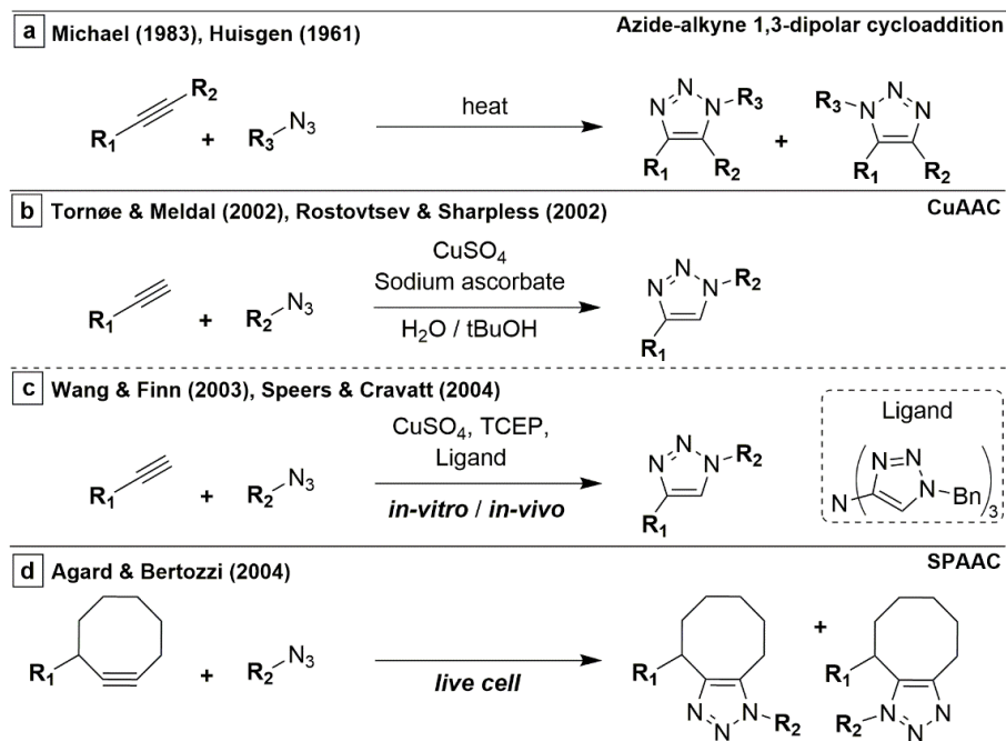
Scheme 12: Overview of the azide-alkyne 1,3-dipolar cycloaddition, CuAAC and SPAAC reactions.
