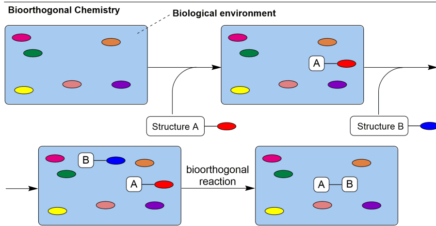
Figure 1: A representation of bioorthogonal chemistry: (1) the biological environment to which (2) structure A with a “red” bioorthogonal group is added, and then (3) structure B with a “blue” bioorthogonal group is added, after which (4) structures with “red” and “blue” bioorthogonal groups react with each other without affecting the biological environment.
