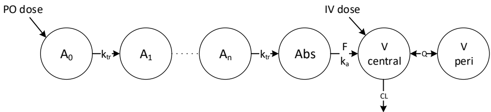
Figure S1: Structure of the pharmacokinetic model
