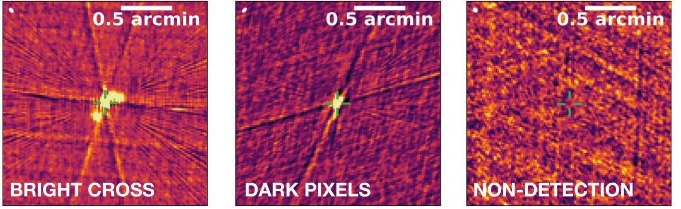
Figure 3. An illustration of two artifact types and a NON-DETECTION source in VLASS images. The algorithm identifies cross pattern and dark pixel artifacts, assigning appropriate quality flag values (1 for cross pattern presence, 2 for dark pixel presence, and 3 for both artifacts in the image). Sources with low S/Ns that are difficult to discern by visual inspection are classified as NON-DETECTION sources.
