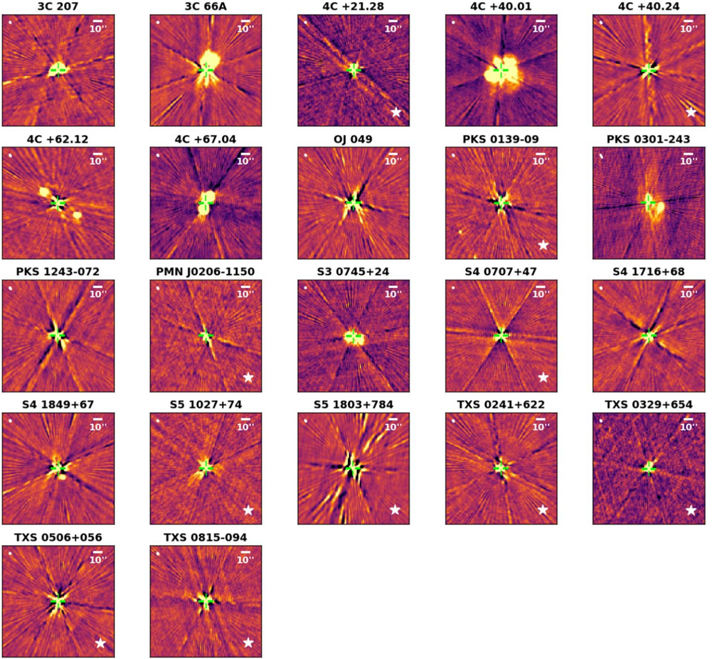
Figure 11. VLASS2 images for 22 MOJAVE blazars classified as likely non-blazars. Each source has undergone visual inspection, and any discrepancies (are COMPACT instead of NON-COMPACT) found during this process are indicated by a visual flag in the resulting table. For each of these sources, our revised visual classification is provided. These revised sources are marked with a white star on their image.
