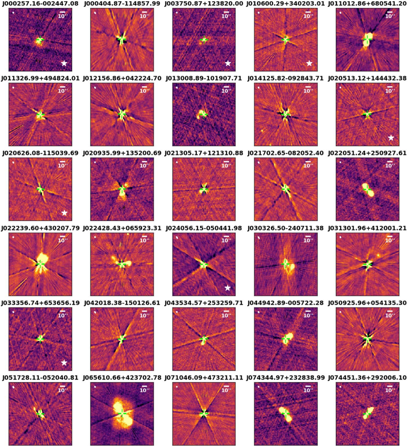
Figure 7. Same as Figure 5 but for 2-SIDE EXTENDED sources in Roma-BzCAT.
