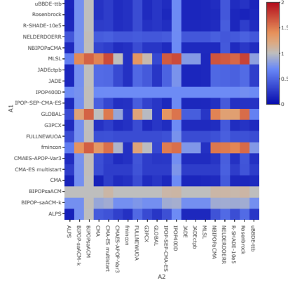
Figure 5.5: Relative ERT of configuration switches relative to \text{VBS}_{\text{static}} , for 10-dimensional function 21. The X- and Y-axes indicate algorithms selected as A_2 and A_1 respectively. Larger values (red) indicate better algorithm combinations.
