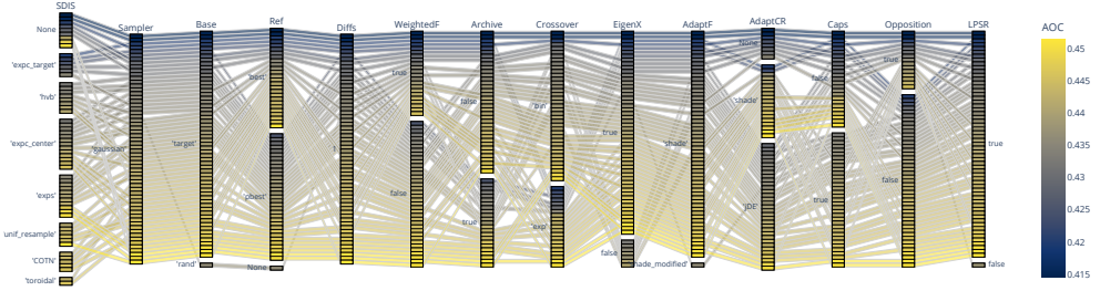
Figure 4.6: Parallel coordinate plot showing the modules activated in the elite configuration found across 10 runs of irace, on F19 in 5D. Configurations are colored based on normalized AOC.
