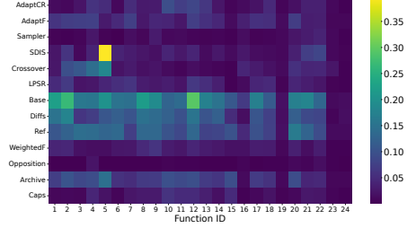
Figure 4.2: Importance of each module to the AOC on each of the 24 BBOB functions, aggregated over the used dimensions. Importance is calculated as the sum of absolute values from Figures 4.1a and 4.1b.
