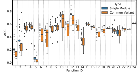
Figure 4.3: Performance distribution (AOC) of the 30 single-module DE variants and the 11 common DE variants from Table 4.3, for the 10-dimensional BBOB problems.
